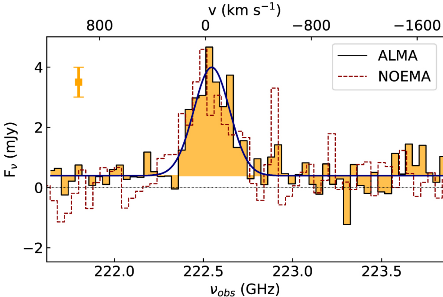
Figure 1. from The z = 7.54 Quasar ULAS J1342+0928 Is Hosted by a Galaxy Merger null 2019 APJL 881 L23 doi:10.3847/2041-8213/ab3659 http://dx.doi.org/10.3847/2041-8213/ab3659 © 2019. The American Astronomical Society. All rights reserved.
