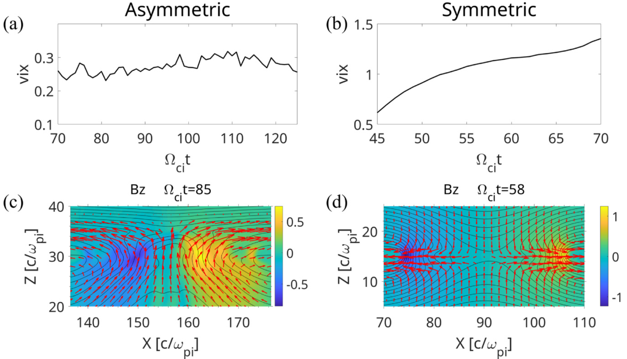
Figure 6. from Reconnection Front Associated with Asymmetric Magnetic Reconnection: Particle-in-cell Simulations null 2019 APJL 881 L22 doi:10.3847/2041-8213/ab3655 http://dx.doi.org/10.3847/2041-8213/ab3655 © 2019. The American Astronomical Society. All rights reserved.
