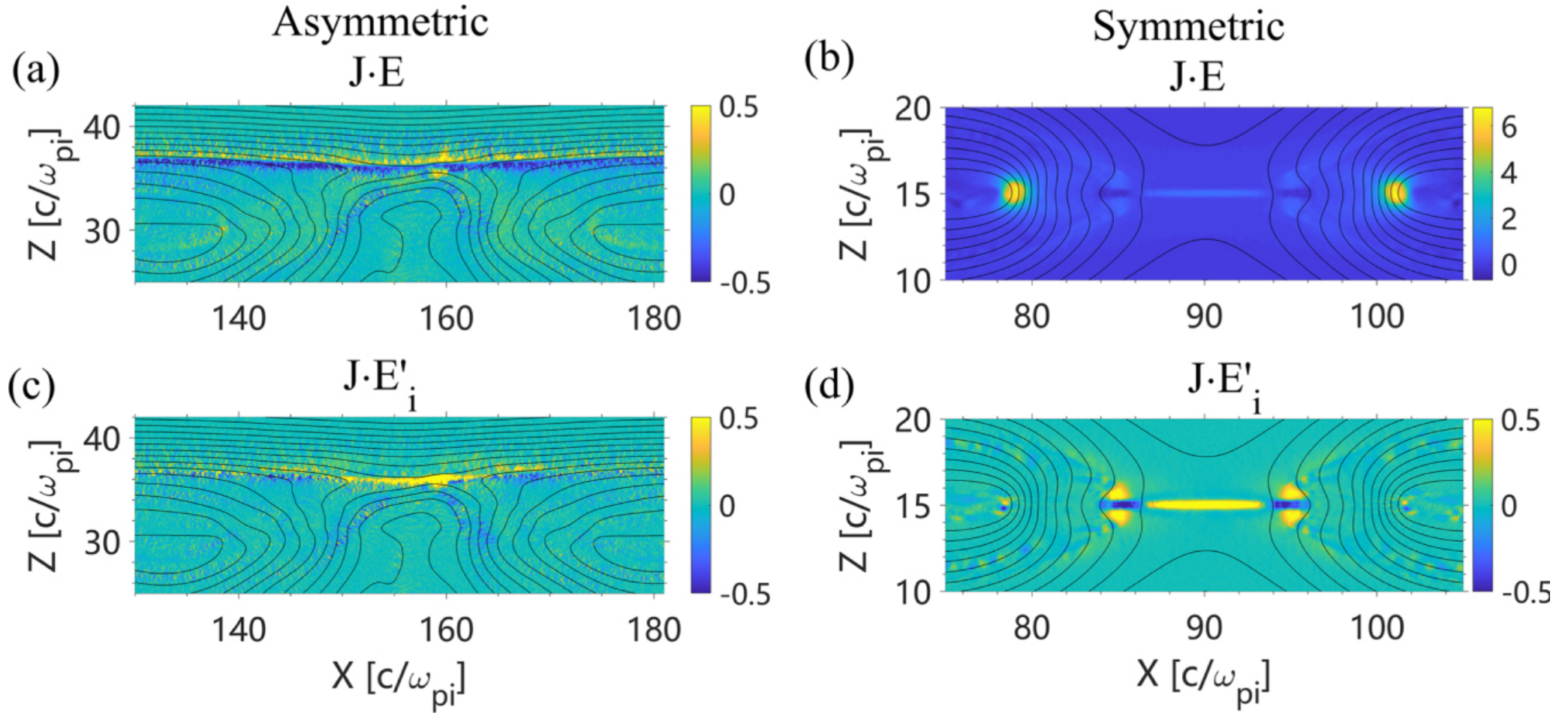
Figure 4. from Reconnection Front Associated with Asymmetric Magnetic Reconnection: Particle-in-cell Simulations null 2019 APJL 881 L22 doi:10.3847/2041-8213/ab3655 http://dx.doi.org/10.3847/2041-8213/ab3655 © 2019. The American Astronomical Society. All rights reserved.
