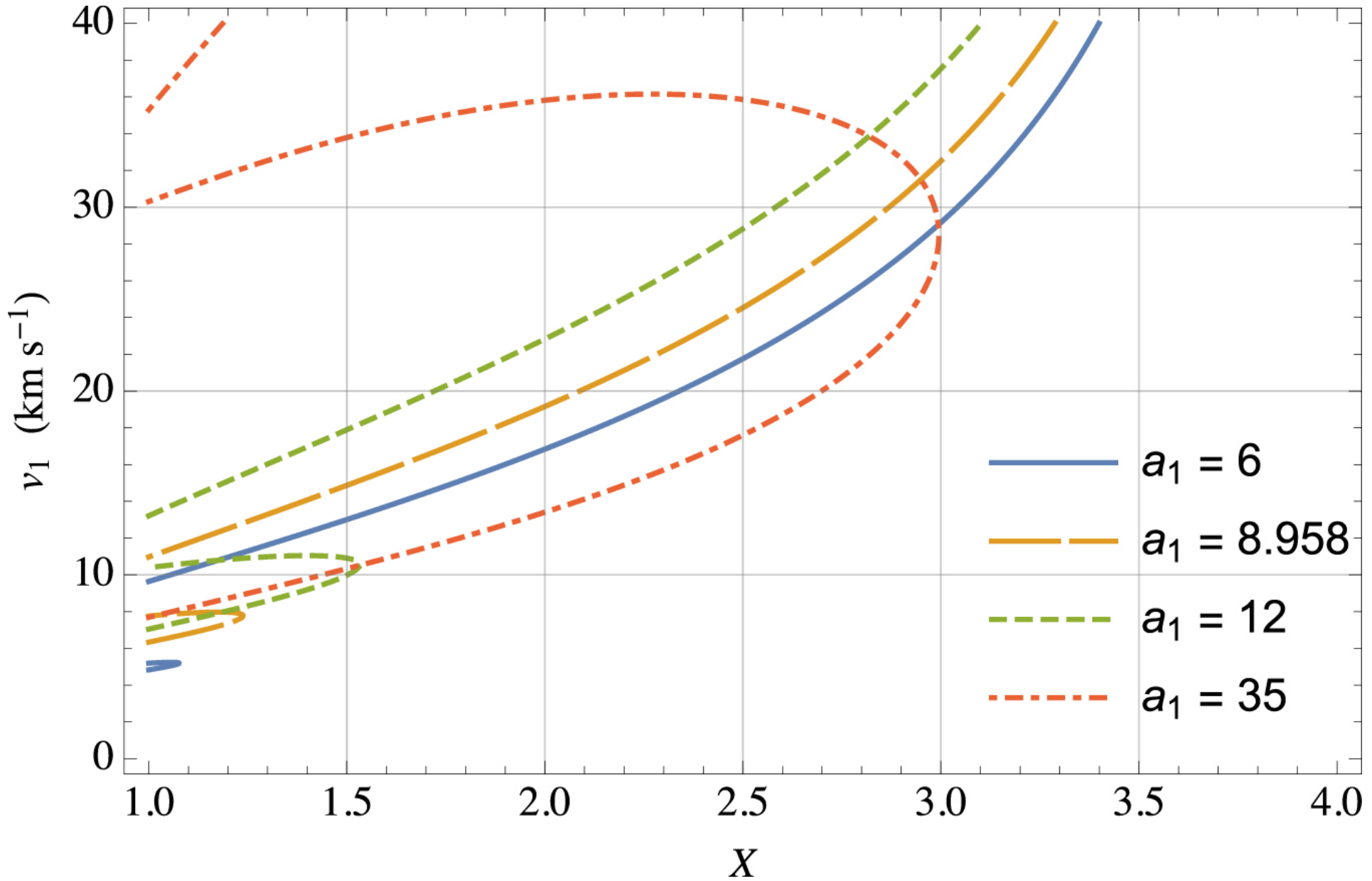
Figure 7. from Smoothing of MHD Shocks in Mode Conversion null 2019 APJL 881 L21 doi:10.3847/2041-8213/ab3423 http://dx.doi.org/10.3847/2041-8213/ab3423 © 2019. The American Astronomical Society. All rights reserved.
