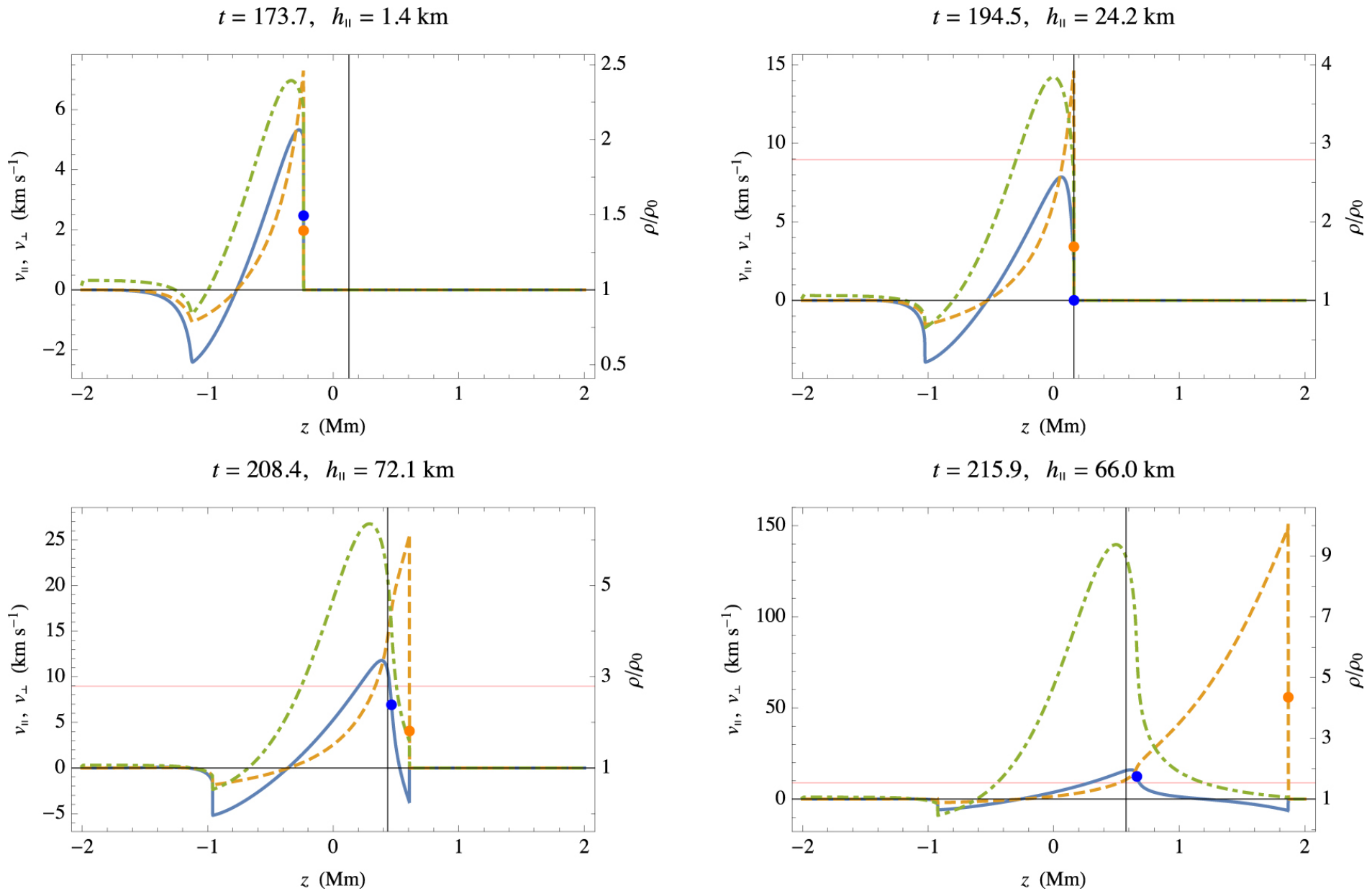
Figure 3. from Smoothing of MHD Shocks in Mode Conversion null 2019 APJL 881 L21 doi:10.3847/2041-8213/ab3423 http://dx.doi.org/10.3847/2041-8213/ab3423 © 2019. The American Astronomical Society. All rights reserved.
