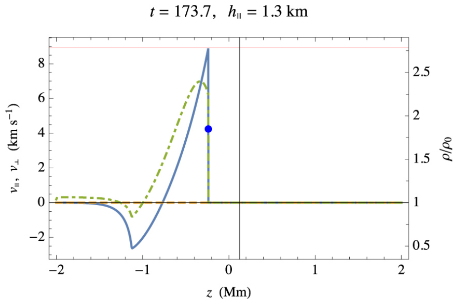
Figure 1. from Smoothing of MHD Shocks in Mode Conversion null 2019 APJL 881 L21 doi:10.3847/2041-8213/ab3423 http://dx.doi.org/10.3847/2041-8213/ab3423 © 2019. The American Astronomical Society. All rights reserved.
