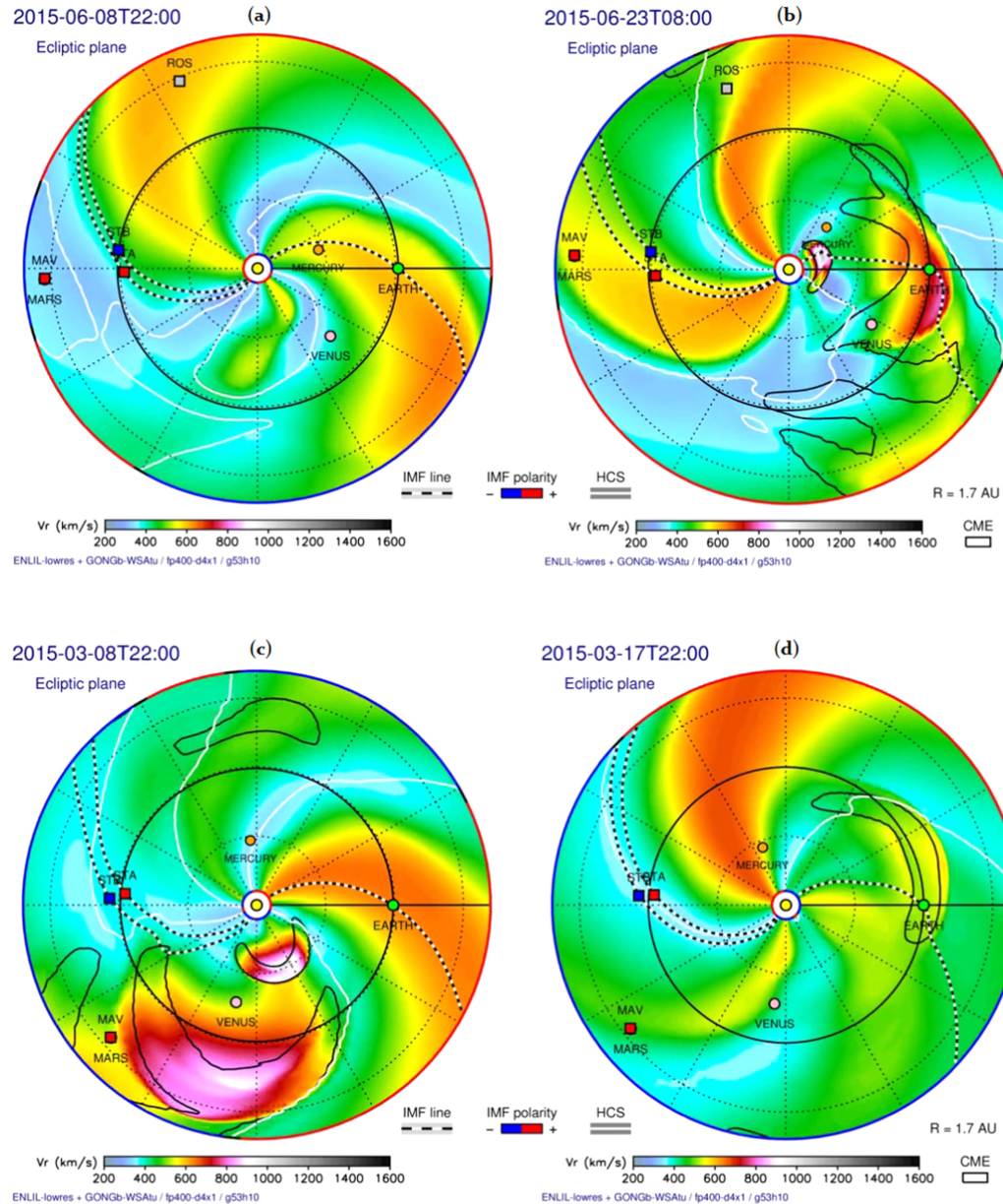
Figure 6. from Acceleration of Energetic Ions in Corotating Interaction Region near 1.5 au: Evidence from MAVEN null 2019 APJL 880 L3 doi:10.3847/2041-8213/ab2b43 https://dx.doi.org/10.3847/2041-8213/ab2b43 © 2019. The American Astronomical Society. All rights reserved.
