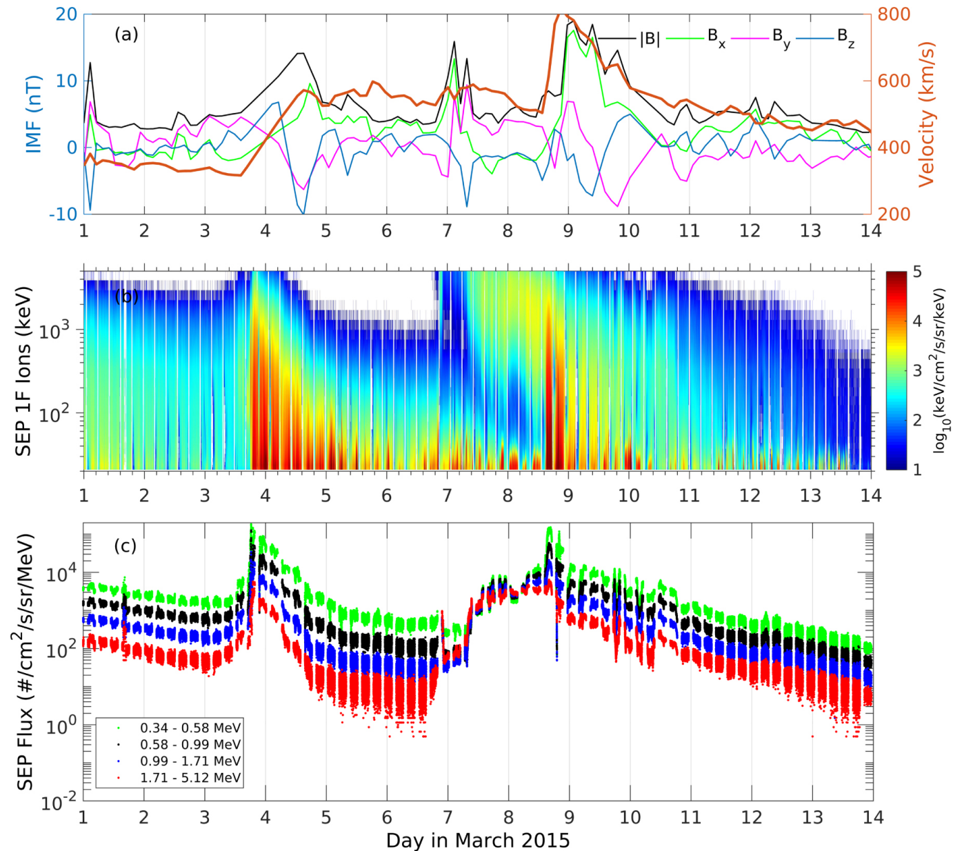
Figure 5. from Acceleration of Energetic Ions in Corotating Interaction Region near 1.5 au: Evidence from MAVEN null 2019 APJL 880 L3 doi:10.3847/2041-8213/ab2b43 https://dx.doi.org/10.3847/2041-8213/ab2b43 © 2019. The American Astronomical Society. All rights reserved.
