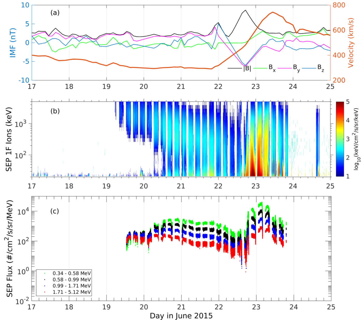
Figure 2. from Acceleration of Energetic Ions in Corotating Interaction Region near 1.5 au: Evidence from MAVEN null 2019 APJL 880 L3 doi:10.3847/2041-8213/ab2b43 https://dx.doi.org/10.3847/2041-8213/ab2b43 © 2019. The American Astronomical Society. All rights reserved.
