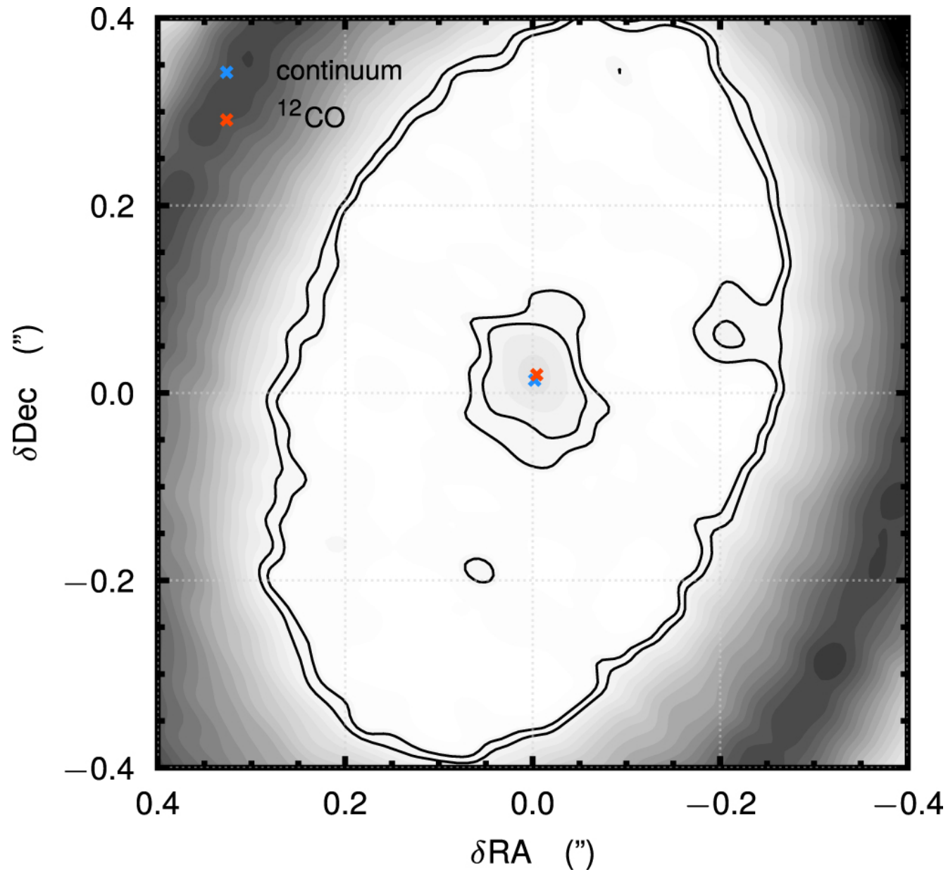
Figure 7. from Detection of Continuum Submillimeter Emission Associated with Candidate Protoplanets null 2019 APJL 879 L25 doi:10.3847/2041-8213/ab2a12 https://dx.doi.org/10.3847/2041-8213/ab2a12 © 2019. The American Astronomical Society. All rights reserved.
