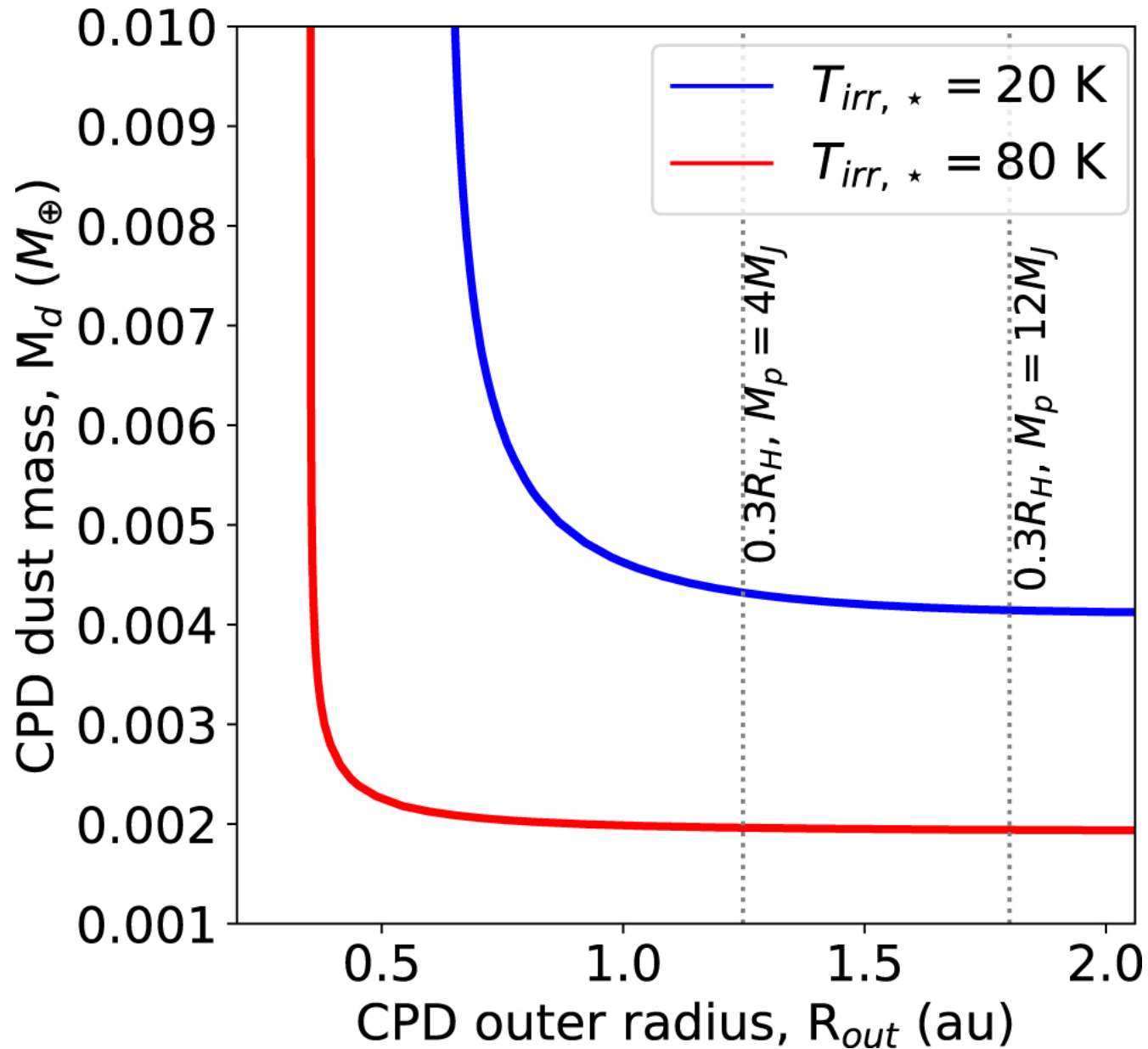
Figure 3. from Detection of Continuum Submillimeter Emission Associated with Candidate Protoplanets null 2019 APJL 879 L25 doi:10.3847/2041-8213/ab2a12 https://dx.doi.org/10.3847/2041-8213/ab2a12 © 2019. The American Astronomical Society. All rights reserved.
