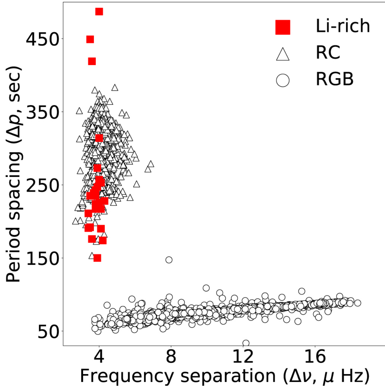
Figure 4. from Survey of Li-rich Giants among Kepler and LAMOST Fields: Determination of Li-rich Giants' Evolutionary Phase null 2019 APJL 878 L21 doi:10.3847/2041-8213/ab2599 http://dx.doi.org/10.3847/2041-8213/ab2599 © 2019. The American Astronomical Society. All rights reserved.
