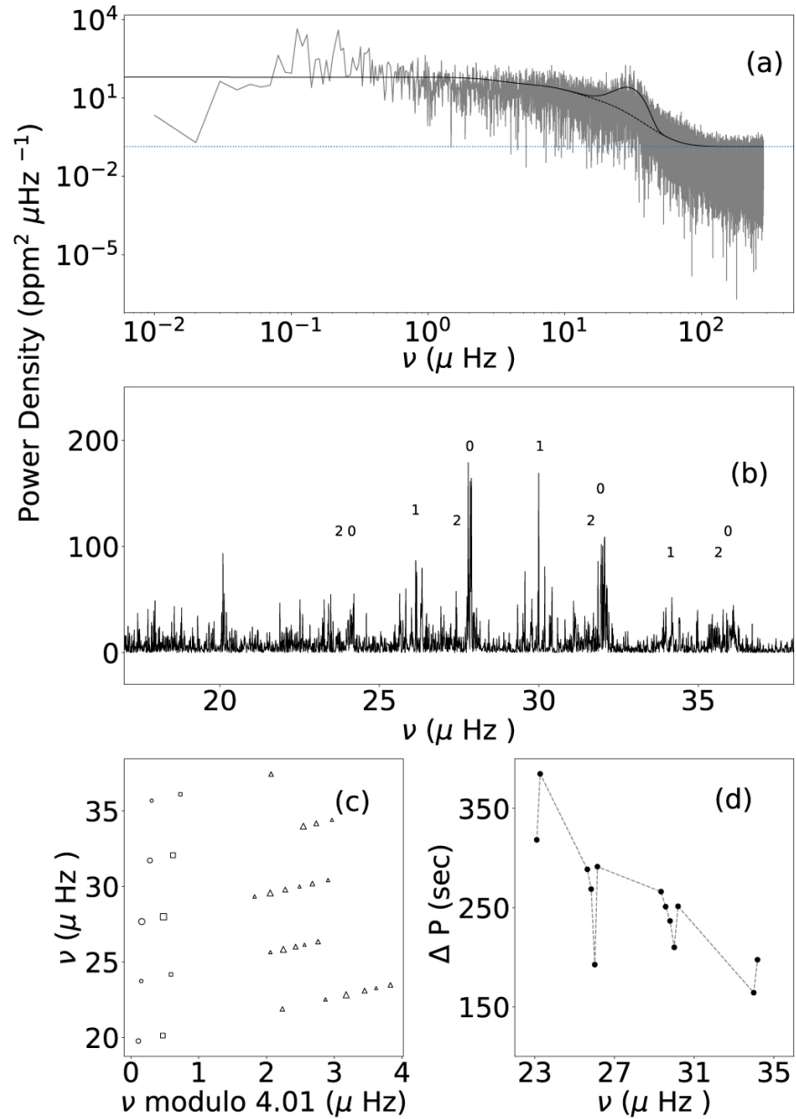
Figure 3. from Survey of Li-rich Giants among Kepler and LAMOST Fields: Determination of Li-rich Giants' Evolutionary Phase null 2019 APJL 878 L21 doi:10.3847/2041-8213/ab2599 http://dx.doi.org/10.3847/2041-8213/ab2599
