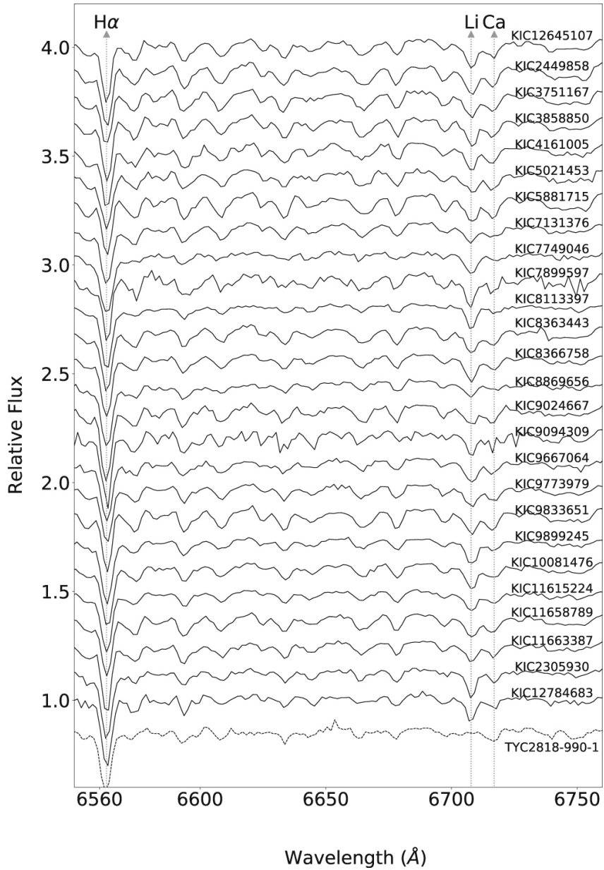
Figure 2. from Survey of Li-rich Giants among Kepler and LAMOST Fields: Determination of Li-rich Giants' Evolutionary Phase null 2019 APJL 878 L21 doi:10.3847/2041-8213/ab2599 http://dx.doi.org/10.3847/2041-8213/ab2599 © 2019. The American Astronomical Society. All rights reserved.
