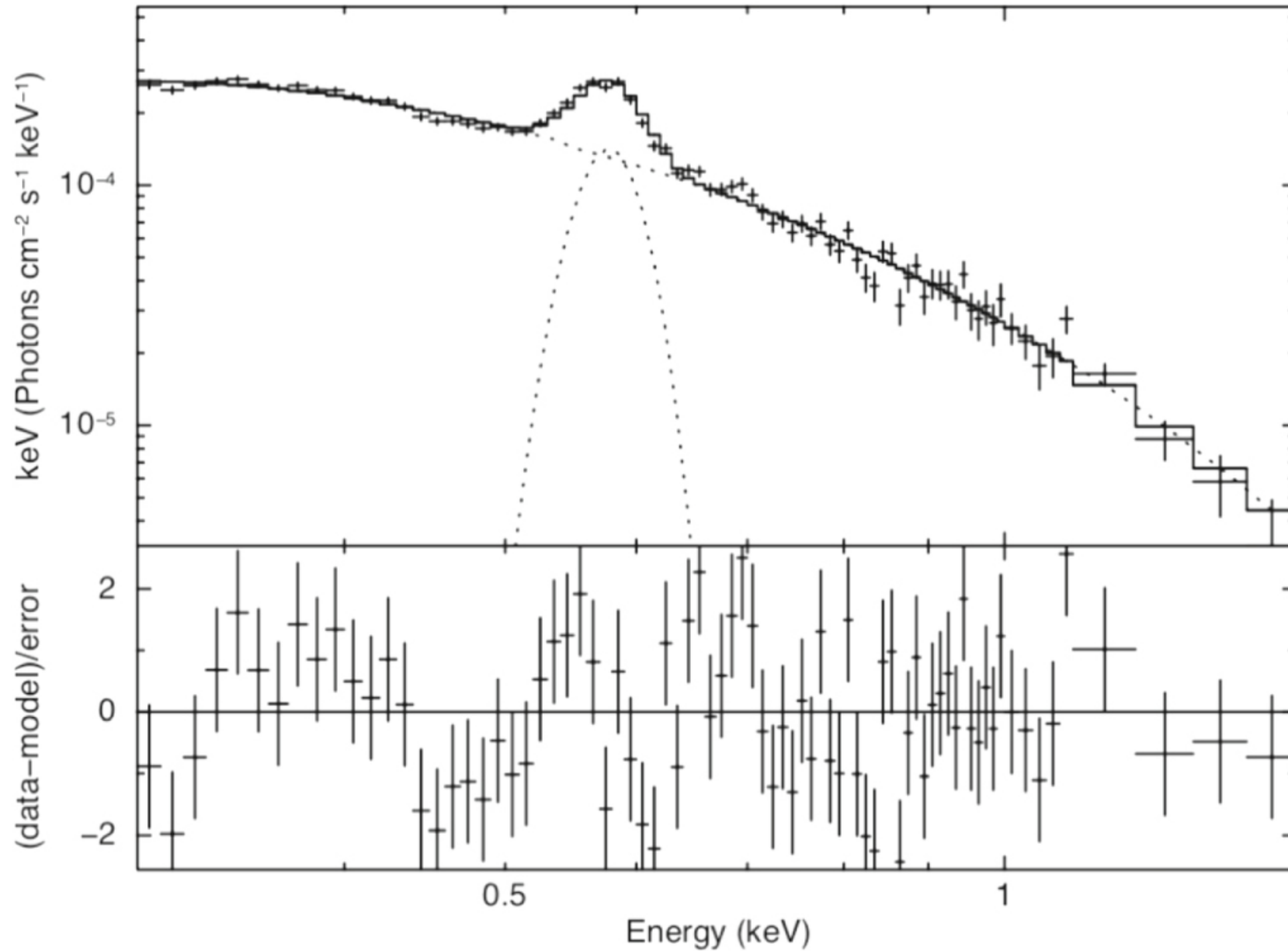
Figure 7. from Discovery of Soft X-Ray Pulsations from PSR J1231–1411 using NICER null 2019 APJL 878 L22 doi:10.3847/2041-8213/ab2539 http://dx.doi.org/10.3847/2041-8213/ab2539 © 2019. The American Astronomical Society. All rights reserved.
