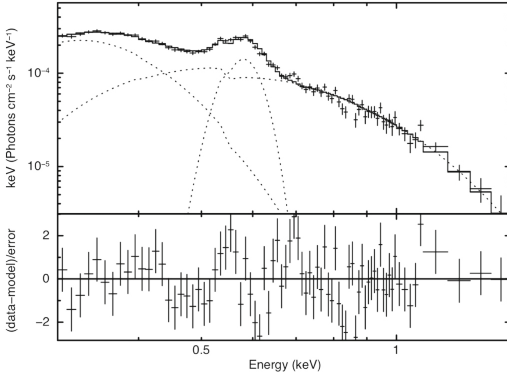
Figure 6. from Discovery of Soft X-Ray Pulsations from PSR J1231–1411 using NICER null 2019 APJL 878 L22 doi:10.3847/2041-8213/ab2539 http://dx.doi.org/10.3847/2041-8213/ab2539 © 2019. The American Astronomical Society. All rights reserved.
