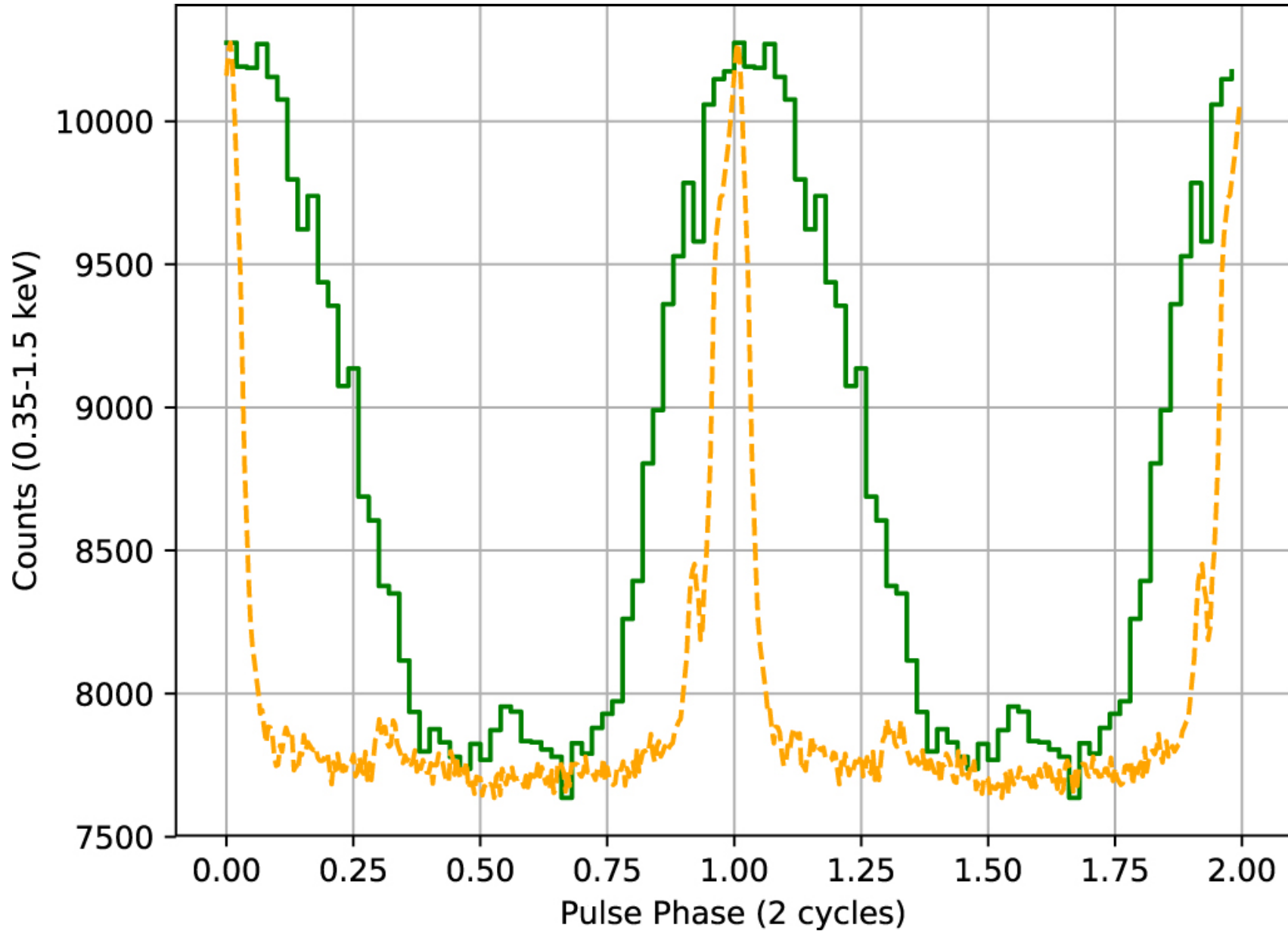
Figure 5. from Discovery of Soft X-Ray Pulsations from PSR J1231–1411 using NICER null 2019 APJL 878 L22 doi:10.3847/2041-8213/ab2539 http://dx.doi.org/10.3847/2041-8213/ab2539 © 2019. The American Astronomical Society. All rights reserved.
