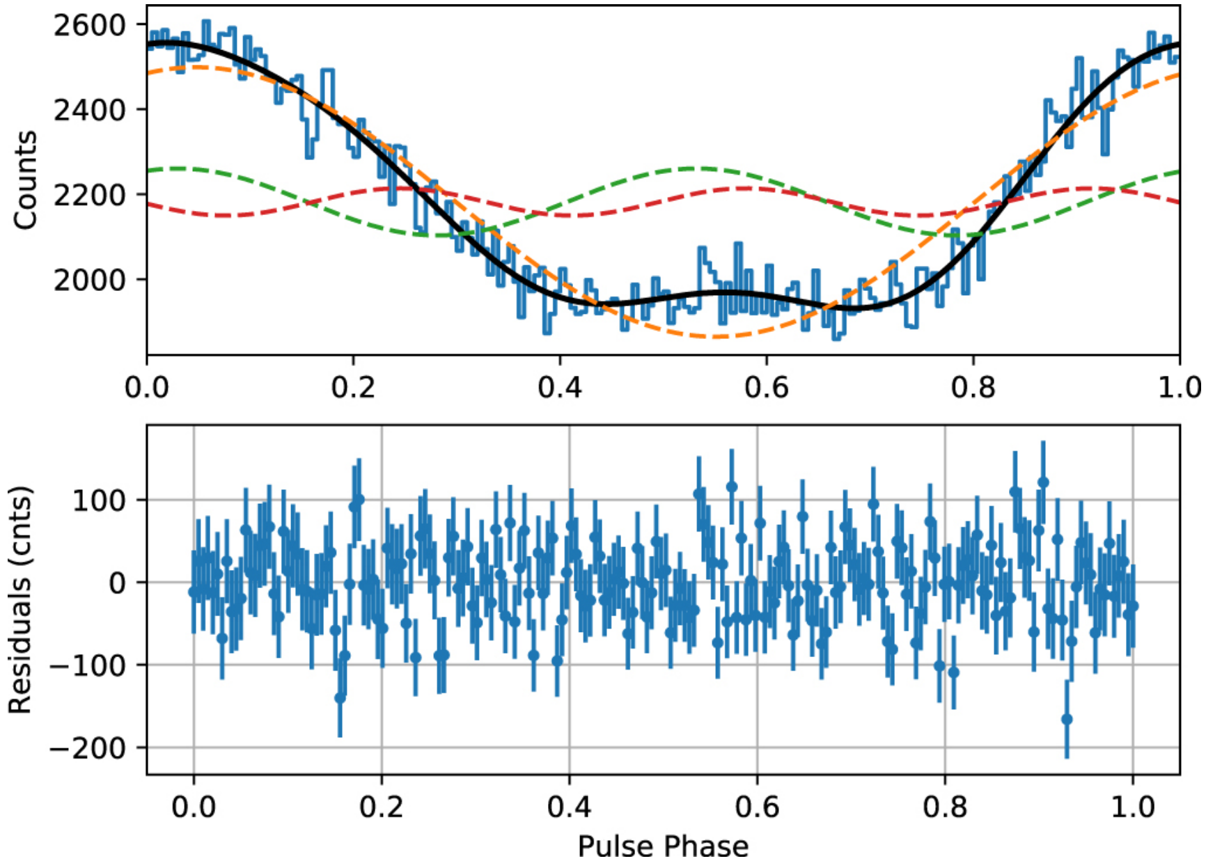
Figure 4. from Discovery of Soft X-Ray Pulsations from PSR J1231–1411 using NICER null 2019 APJL 878 L22 doi:10.3847/2041-8213/ab2539 http://dx.doi.org/10.3847/2041-8213/ab2539 © 2019. The American Astronomical Society. All rights reserved.
