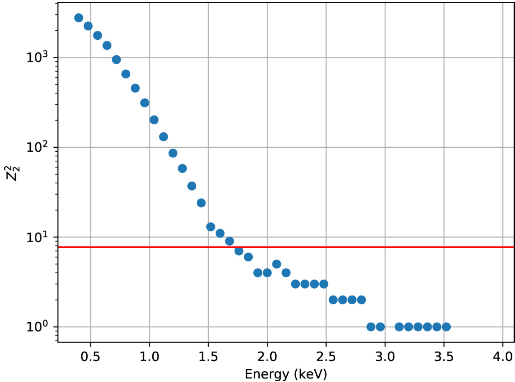
Figure 3. from Discovery of Soft X-Ray Pulsations from PSR J1231–1411 using NICER null 2019 APJL 878 L22 doi:10.3847/2041-8213/ab2539 http://dx.doi.org/10.3847/2041-8213/ab2539 © 2019. The American Astronomical Society. All rights reserved.
