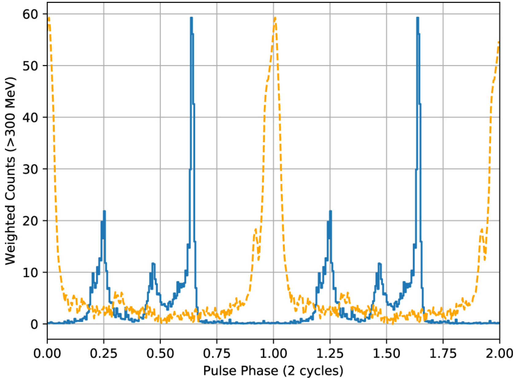
Figure 2. from Discovery of Soft X-Ray Pulsations from PSR J1231–1411 using NICER null 2019 APJL 878 L22 doi:10.3847/2041-8213/ab2539 http://dx.doi.org/10.3847/2041-8213/ab2539 © 2019. The American Astronomical Society. All rights reserved.
