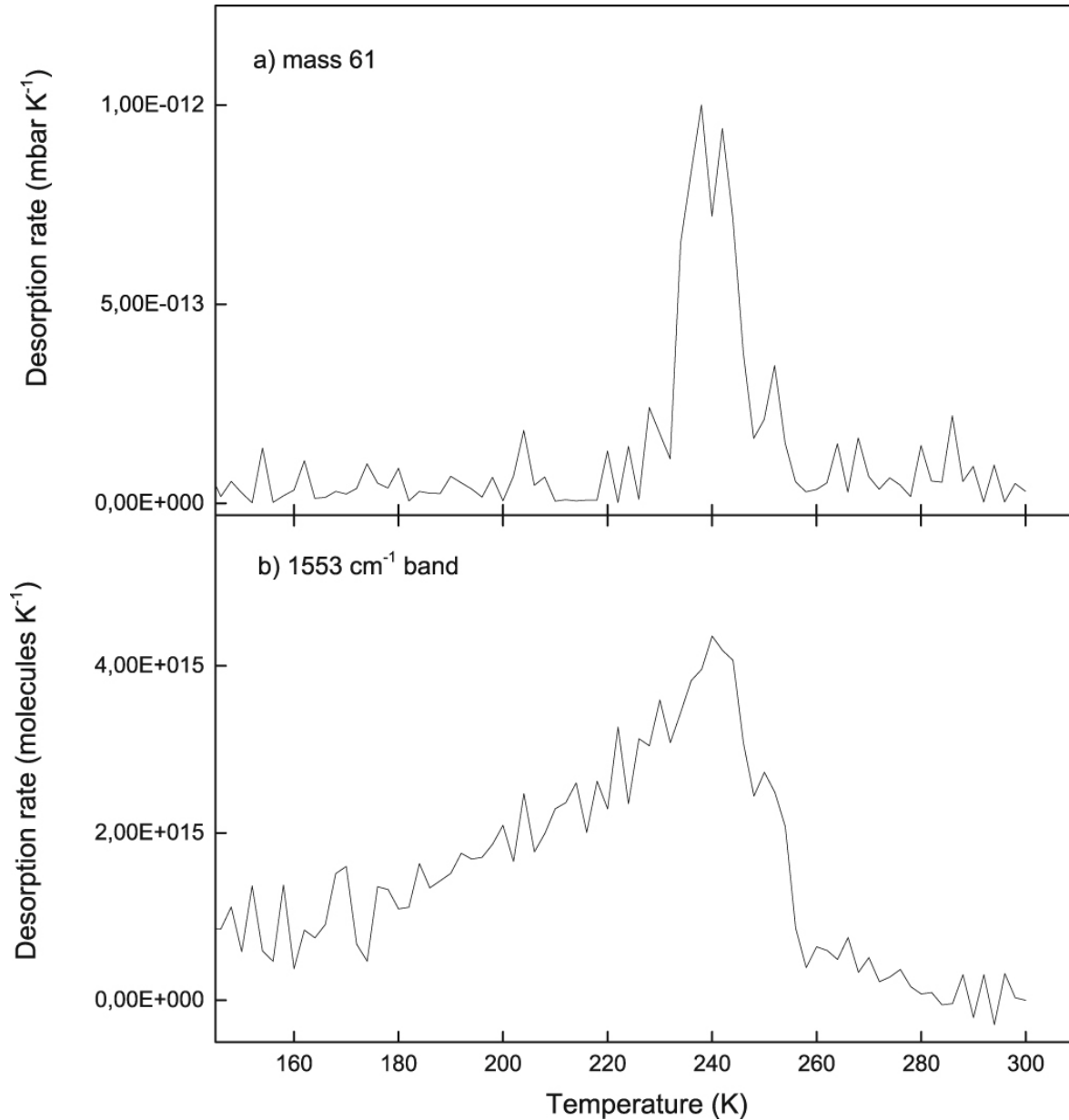
Figure 4. from Evidence of Surface Catalytic Effect on Cosmic Dust Grain Analogs: The Ammonia and Carbon Dioxide Surface Reaction null 2019 APJL 878 L20 doi:10.3847/2041-8213/ab2538 http://dx.doi.org/10.3847/2041-8213/ab2538 © 2019. The American Astronomical Society. All rights reserved.
