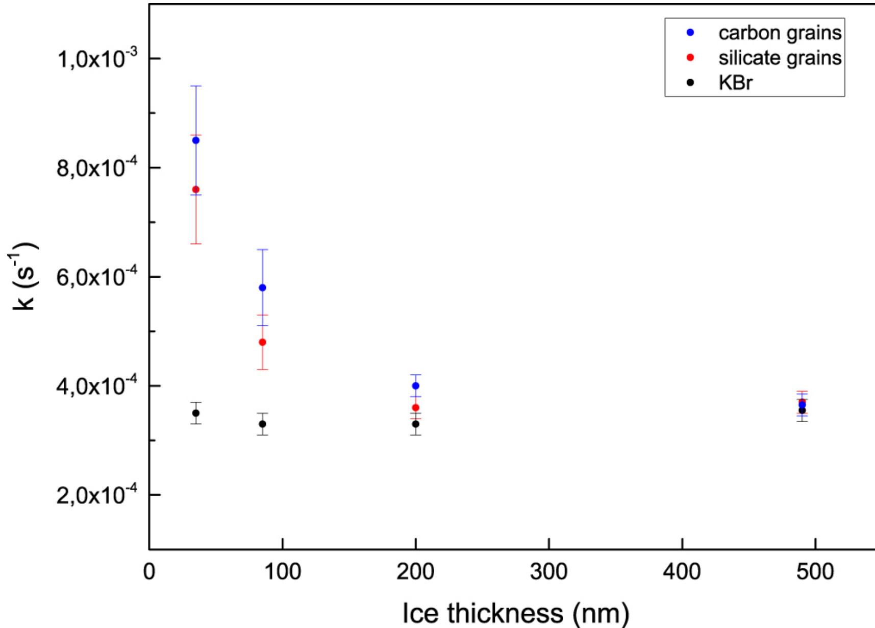
Figure 3. from Evidence of Surface Catalytic Effect on Cosmic Dust Grain Analogs: The Ammonia and Carbon Dioxide Surface Reaction null 2019 APJL 878 L20 doi:10.3847/2041-8213/ab2538 https://dx.doi.org/10.3847/2041-8213/ab2538 © 2019. The American Astronomical Society. All rights reserved.
