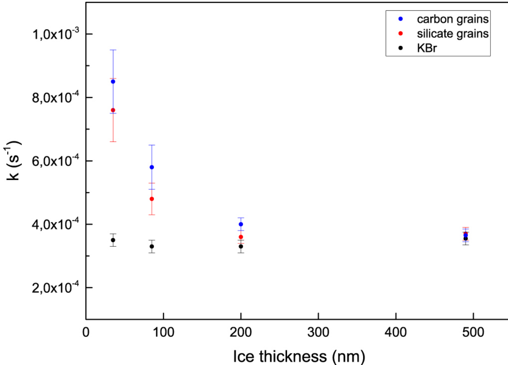
Figure 3. from Evidence of Surface Catalytic Effect on Cosmic Dust Grain Analogs: The Ammonia and Carbon Dioxide Surface Reaction null 2019 APJL 878 L20 doi:10.3847/2041-8213/ab2538 http://dx.doi.org/10.3847/2041-8213/ab2538 © 2019. The American Astronomical Society. All rights reserved.
