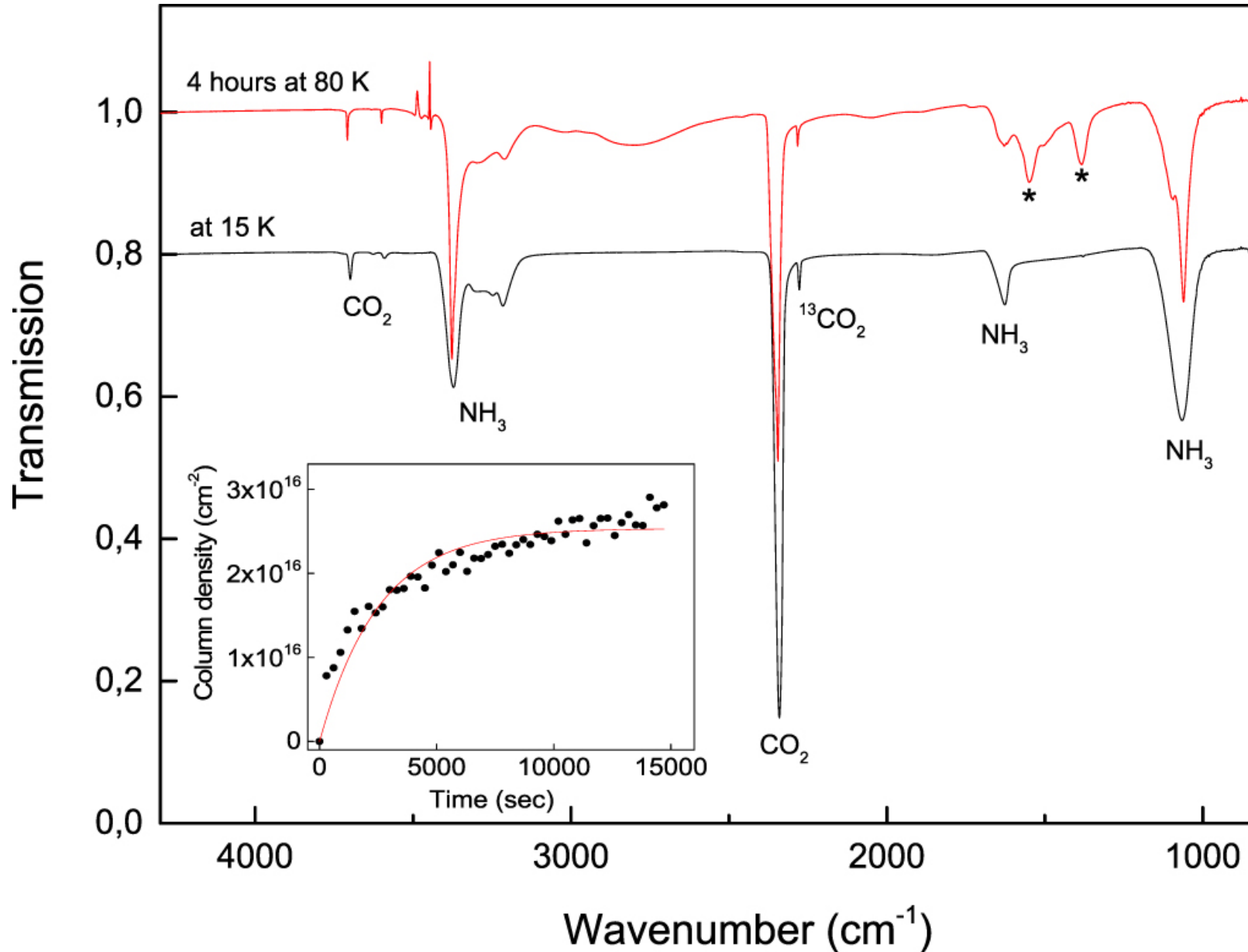
Figure 2. from Evidence of Surface Catalytic Effect on Cosmic Dust Grain Analogs: The Ammonia and Carbon Dioxide Surface Reaction null 2019 APJL 878 L20 doi:10.3847/2041-8213/ab2538 http://dx.doi.org/10.3847/2041-8213/ab2538 © 2019. The American Astronomical Society. All rights reserved.
