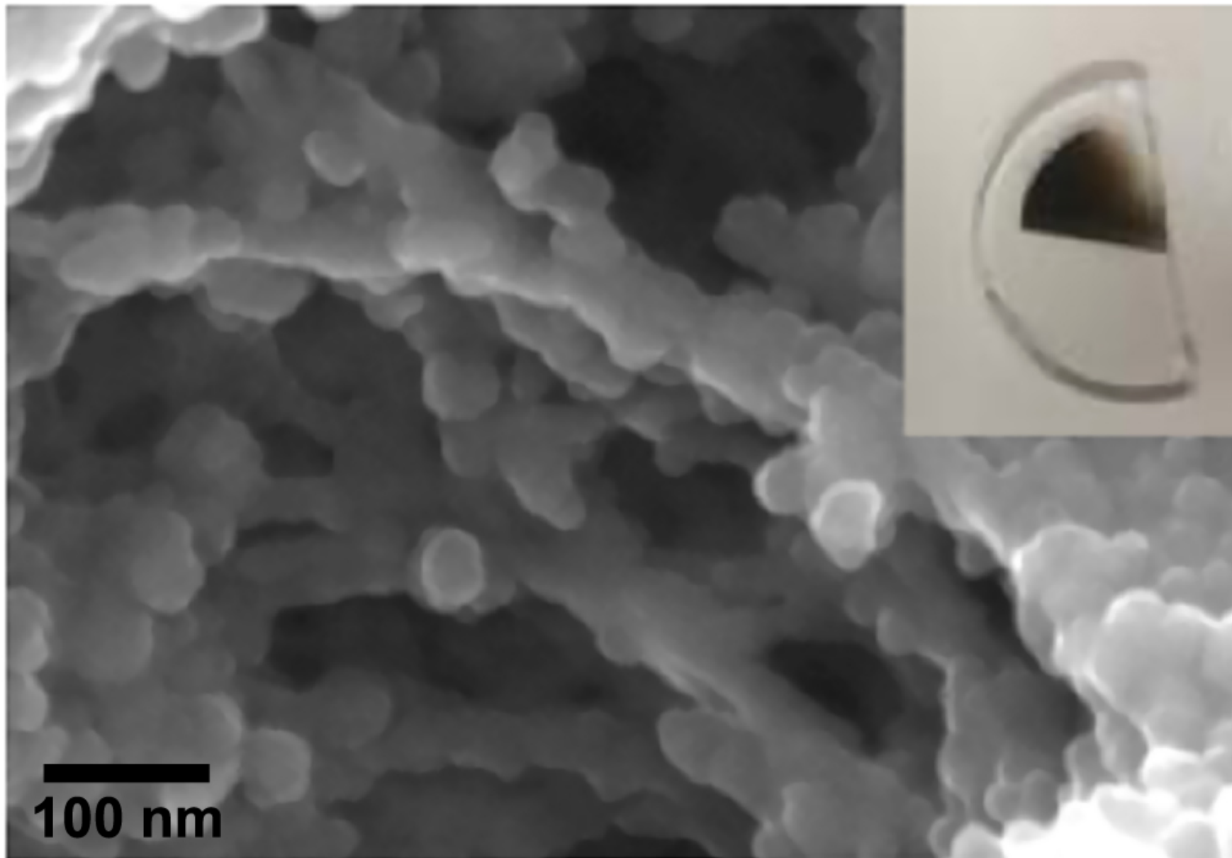
Figure 1. from Evidence of Surface Catalytic Effect on Cosmic Dust Grain Analogs: The Ammonia and Carbon Dioxide Surface Reaction null 2019 APJL 878 L20 doi:10.3847/2041-8213/ab2538 http://dx.doi.org/10.3847/2041-8213/ab2538 © 2019. The American Astronomical Society. All rights reserved.
