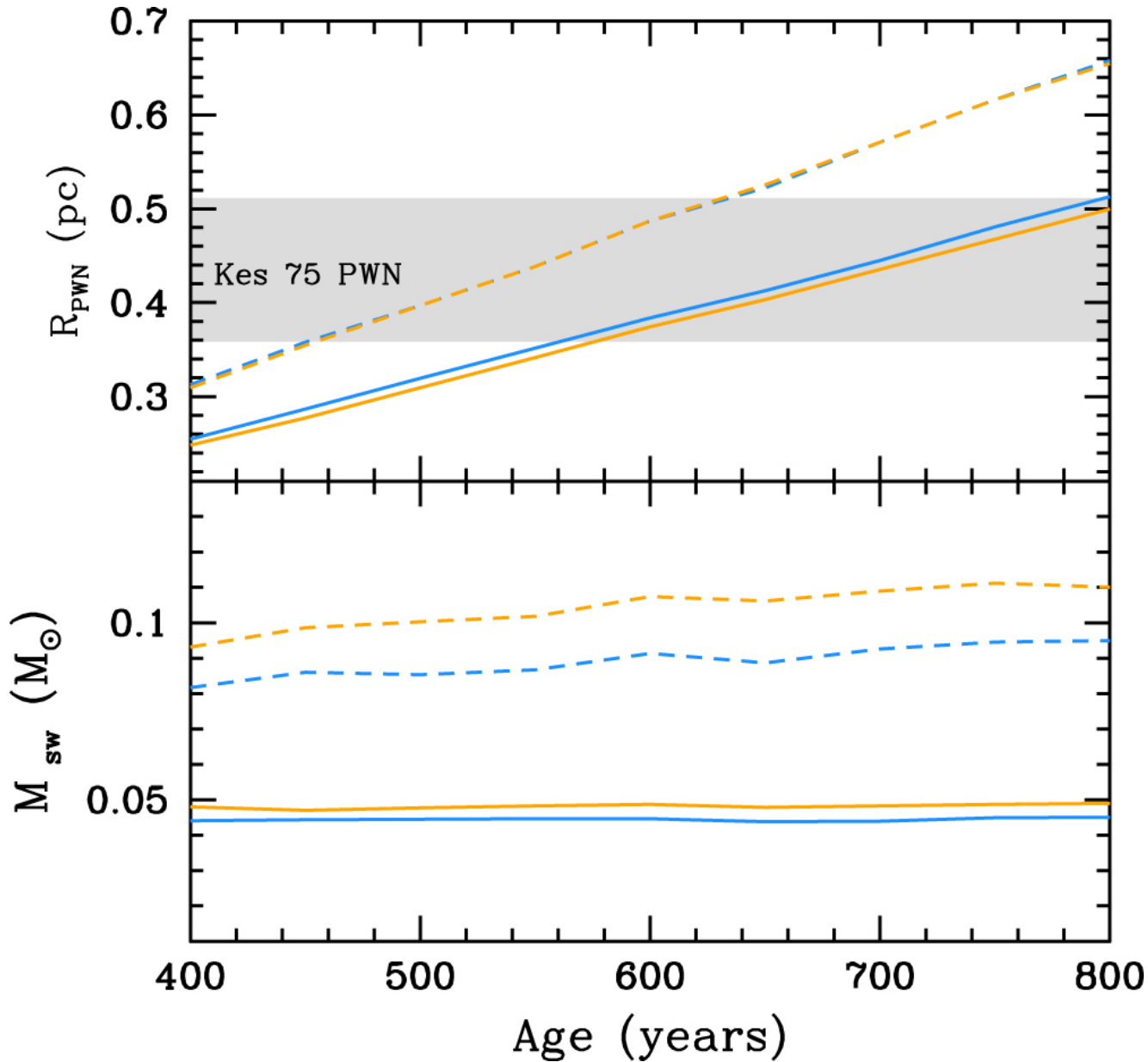
Figure 6. from Probing the Innermost Ejecta Layers in Supernova Remnant Kes 75: Implications for the Supernova Progenitor null 2019 APJL 878 L19 doi:10.3847/2041-8213/ab237c http://dx.doi.org/10.3847/2041-8213/ab237c © 2019. The American Astronomical Society. All rights reserved.
