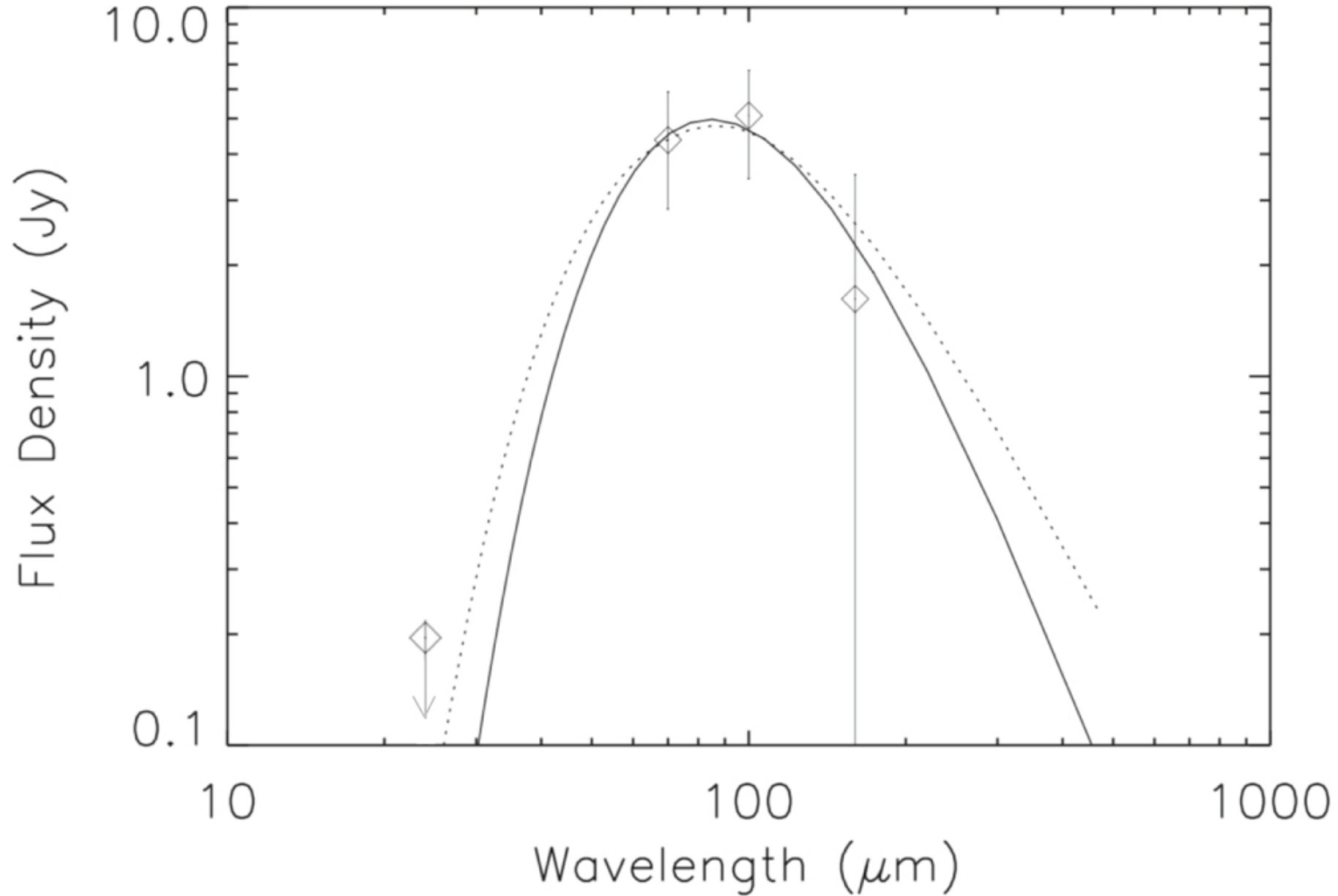
Figure 5. from Probing the Innermost Ejecta Layers in Supernova Remnant Kes 75: Implications for the Supernova Progenitor null 2019 APJL 878 L19 doi:10.3847/2041-8213/ab237c http://dx.doi.org/10.3847/2041-8213/ab237c © 2019. The American Astronomical Society. All rights reserved.
