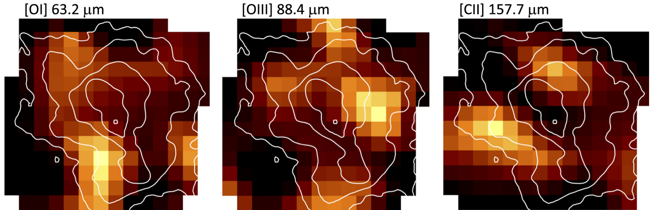
Figure 4. from Probing the Innermost Ejecta Layers in Supernova Remnant Kes 75: Implications for the Supernova Progenitor null 2019 APJL 878 L19 doi:10.3847/2041-8213/ab237c http://dx.doi.org/10.3847/2041-8213/ab237c
