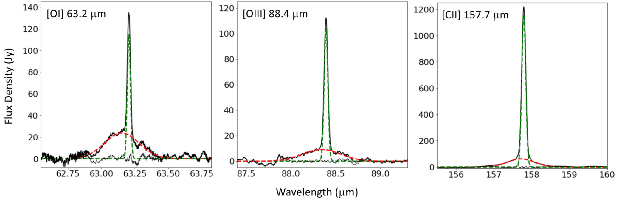
Figure 3. from Probing the Innermost Ejecta Layers in Supernova Remnant Kes 75: Implications for the Supernova Progenitor null 2019 APJL 878 L19 doi:10.3847/2041-8213/ab237c http://dx.doi.org/10.3847/2041-8213/ab237c
