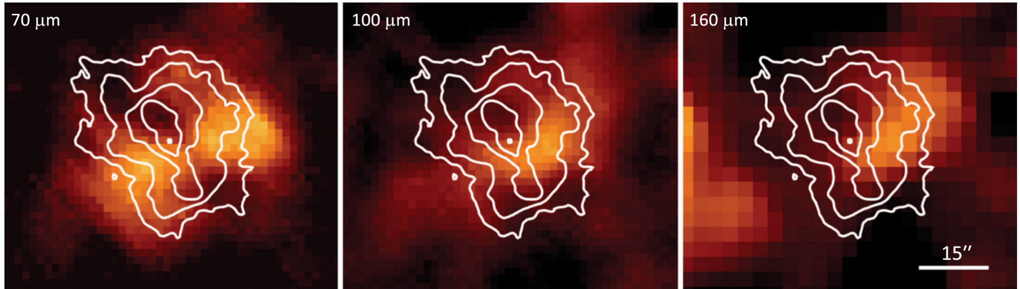
Figure 2. from Probing the Innermost Ejecta Layers in Supernova Remnant Kes 75: Implications for the Supernova Progenitor null 2019 APJL 878 L19 doi:10.3847/2041-8213/ab237c http://dx.doi.org/10.3847/2041-8213/ab237c © 2019. The American Astronomical Society. All rights reserved.
