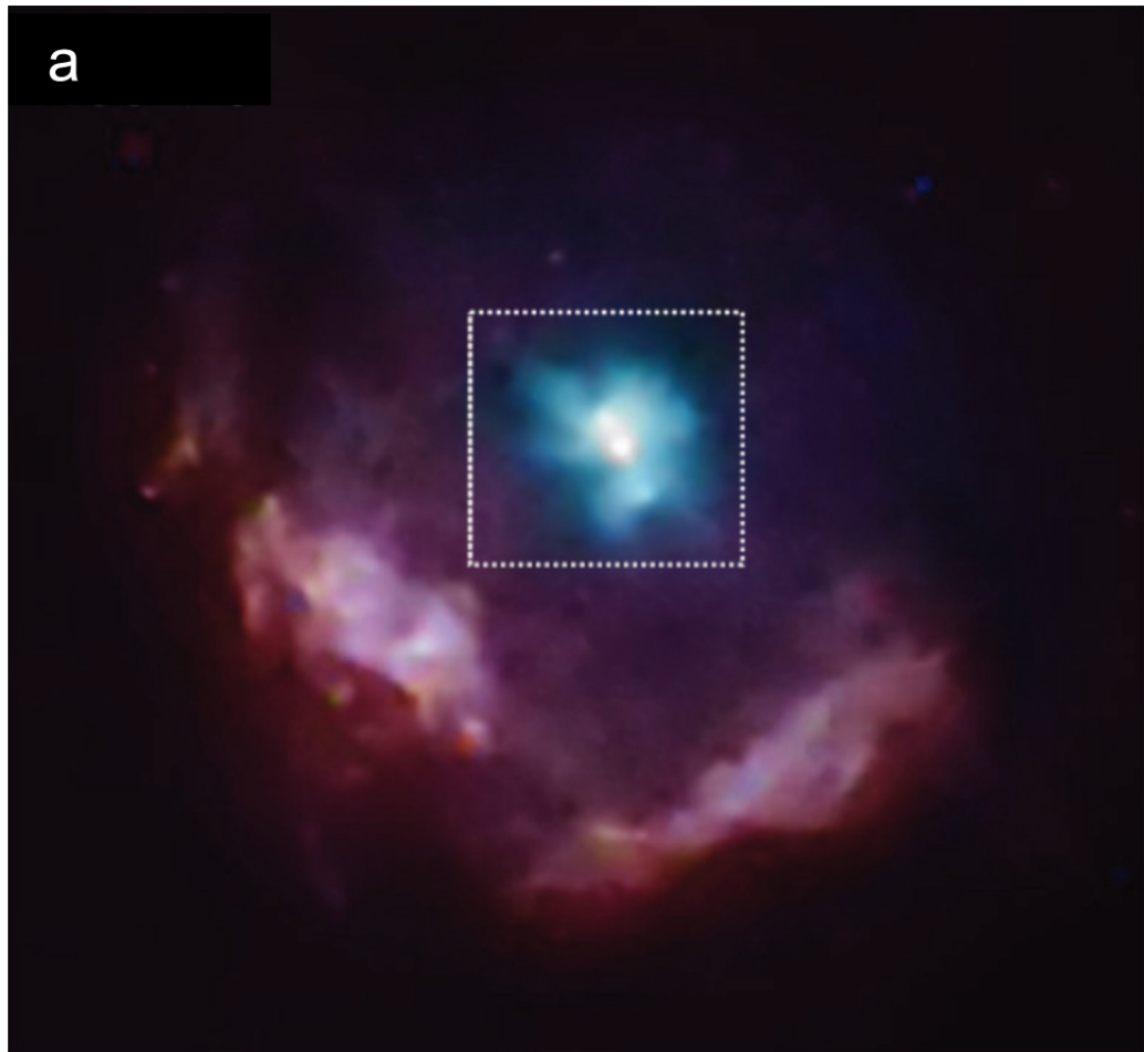
Figure 1. from Probing the Innermost Ejecta Layers in Supernova Remnant Kes 75: Implications for the Supernova Progenitor null 2019 APJL 878 L19 doi:10.3847/2041-8213/ab237c http://dx.doi.org/10.3847/2041-8213/ab237c © 2019. The American Astronomical Society. All rights reserved.
