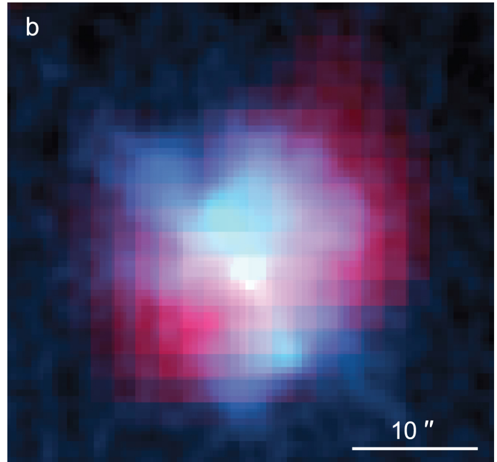
Figure 1. from Probing the Innermost Ejecta Layers in Supernova Remnant Kes 75: Implications for the Supernova Progenitor null 2019 APJL 878 L19 doi:10.3847/2041-8213/ab237c http://dx.doi.org/10.3847/2041-8213/ab237c © 2019. The American Astronomical Society. All rights reserved.
