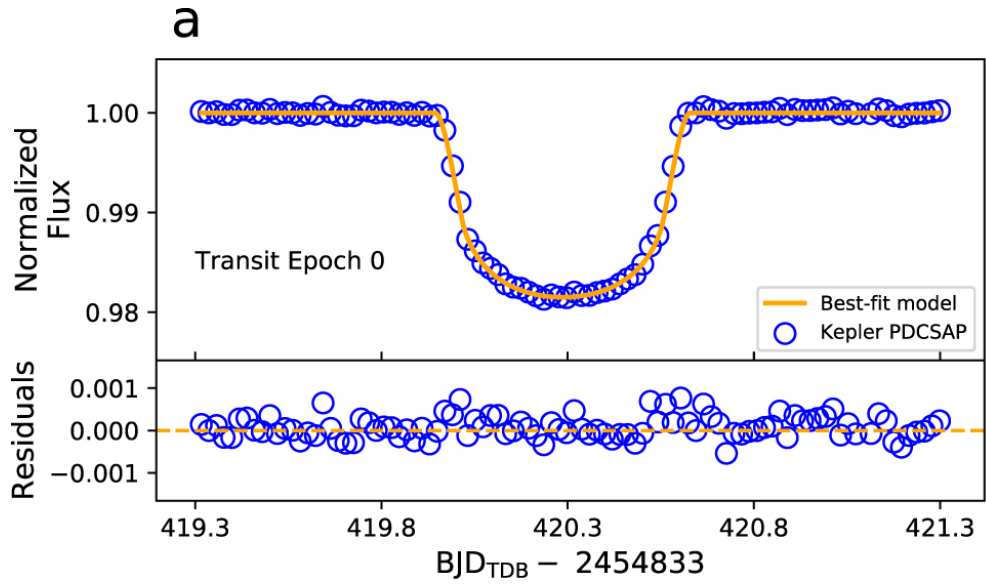
Figure 3. from Spitzer Detection of the Transiting Jupiter-analog Exoplanet Kepler-167e null 2019 APJL 873 L17 doi:10.3847/2041-8213/ab0bb4 http://dx.doi.org/10.3847/2041-8213/ab0bb4 © 2019. The American Astronomical Society. All rights reserved.
