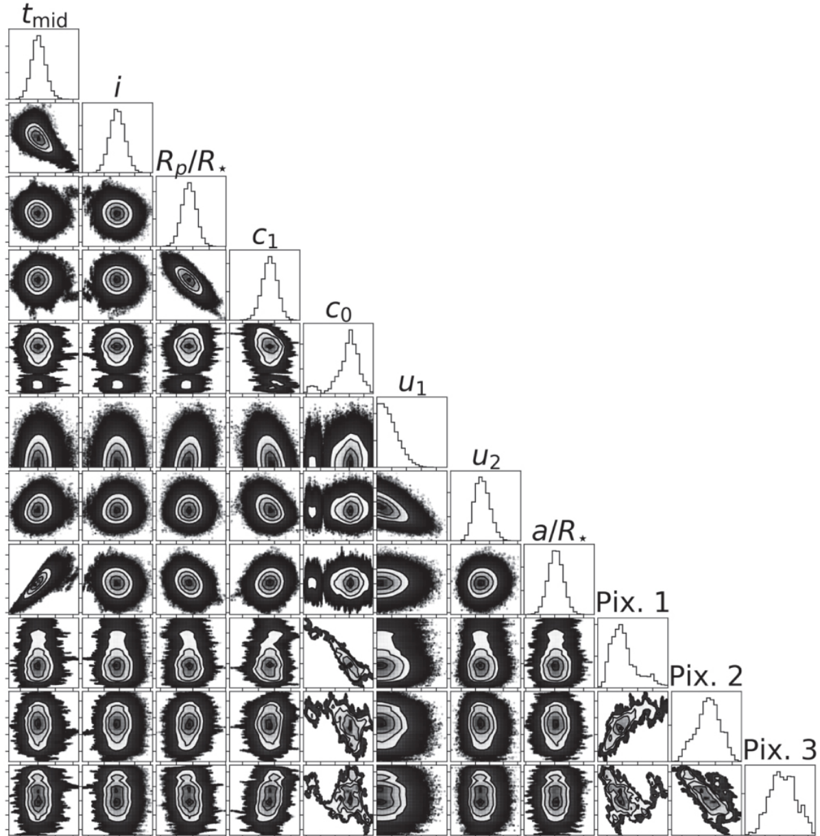
Figure 2. from Spitzer Detection of the Transiting Jupiter-analog Exoplanet Kepler-167e null 2019 APJL 873 L17 doi:10.3847/2041-8213/ab0bb4 http://dx.doi.org/10.3847/2041-8213/ab0bb4 © 2019. The American Astronomical Society. All rights reserved.
