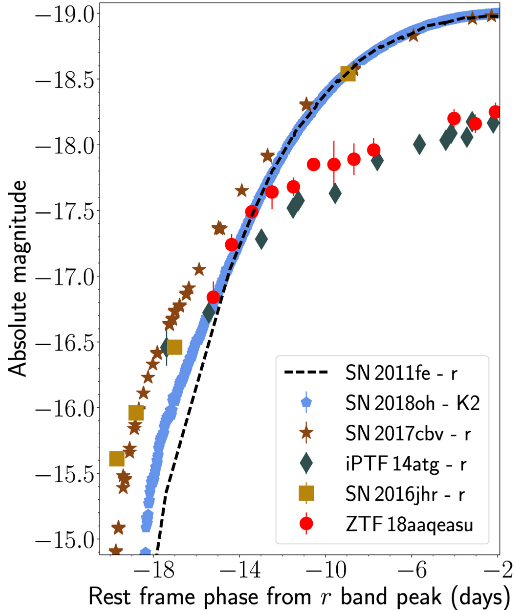
Figure 7. from ZTF 18aaq easu (SN2018byg): A Massive Helium-shell Double Detonation on a Sub-Chandrasekhar-mass White Dwarf null 2019 APJL 873 L18 doi:10.3847/2041-8213/ab0aec http://dx.doi.org/10.3847/2041-8213/ab0aec
