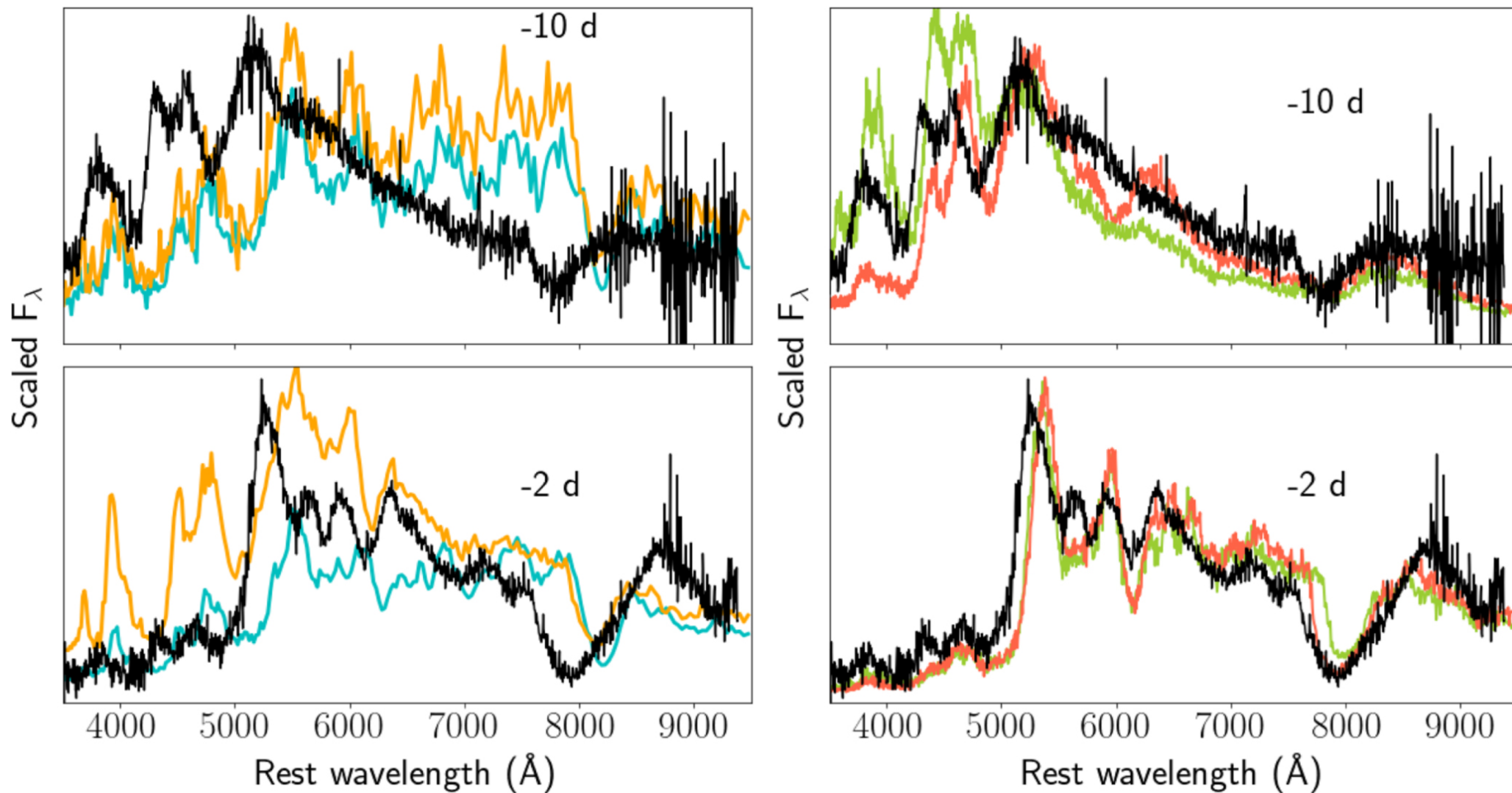
Figure 6. from ZTF 18aaqasu (SN2018byg): A Massive Helium-shell Double Detonation on a Sub-Chandrasekhar-mass White Dwarf null 2019 APJL 873 L18 doi:10.3847/2041-8213/ab0aec https://dx.doi.org/10.3847/2041-8213/ab0aec © 2019. The American Astronomical Society. All rights reserved.
