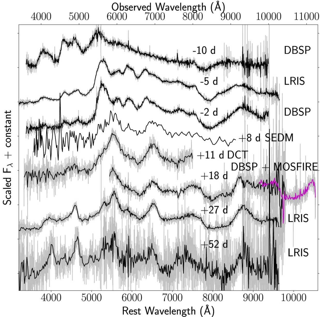
Figure 2. from ZTF 18aaqesu (SN2018byg): A Massive Helium-shell Double Detonation on a Sub-Chandrasekhar-mass White Dwarf null 2019 APJL 873 L18 doi:10.3847/2041-8213/ab0aec http://dx.doi.org/10.3847/2041-8213/ab0aec © 2019. The American Astronomical Society. All rights reserved.
