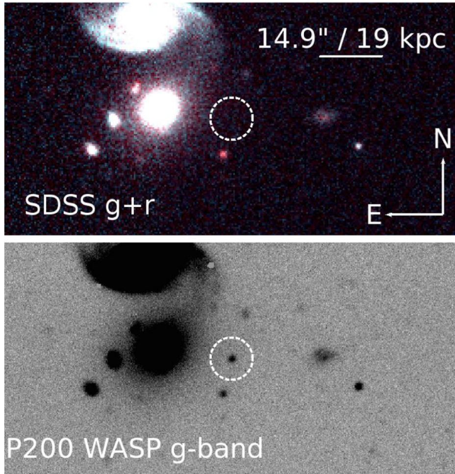
Figure 1. from ZTF 18aaq easu (SN2018byg): A Massive Helium-shell Double Detonation on a Sub-Chandrasekhar-mass White Dwarf null 2019 APJL 873 L18 doi:10.3847/2041-8213/ab0aec http://dx.doi.org/10.3847/2041-8213/ab0aec © 2019. The American Astronomical Society. All rights reserved.
