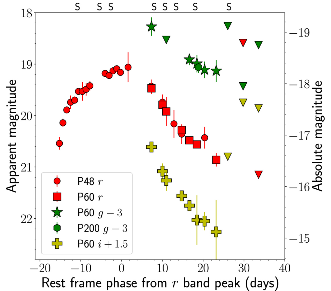
Figure 1. from ZTF 18aaq easu (SN2018byg): A Massive Helium-shell Double Detonation on a Sub-Chandrasekhar-mass White Dwarf null 2019 APJL 873 L18 doi:10.3847/2041-8213/ab0aec http://dx.doi.org/10.3847/2041-8213/ab0aec © 2019. The American Astronomical Society. All rights reserved.
