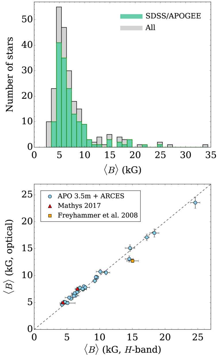
Figure 2. from Discovery of Resolved Magnetically Split Lines in SDSS/APOGEE Spectra of 157 Ap/Bp Stars null 2019 APJL 873 L5 doi:10.3847/2041-8213/ab0750 http://dx.doi.org/10.3847/2041-8213/ab0750 © 2019. The American Astronomical Society. All rights reserved.
