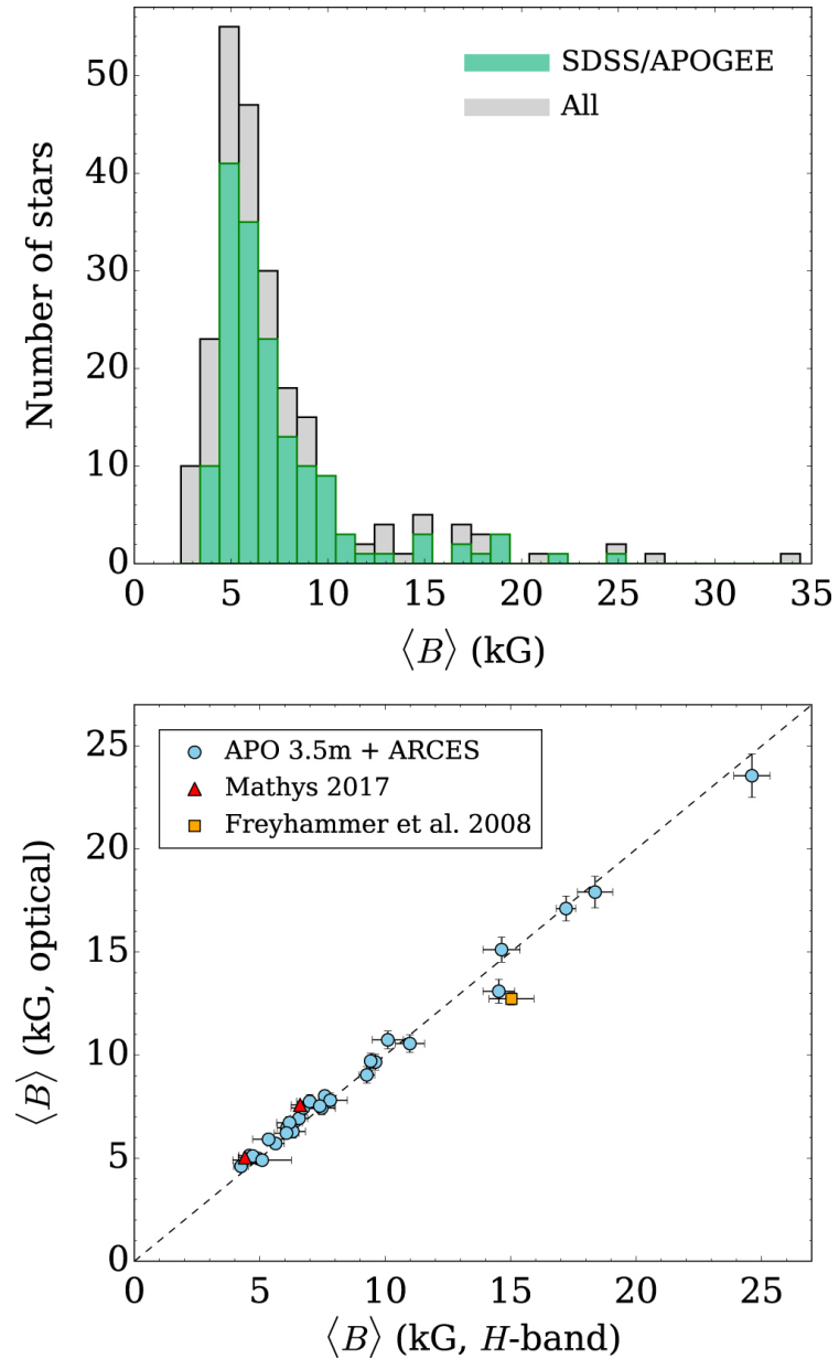
Figure 2. from Discovery of Resolved Magnetically Split Lines in SDSS/APOGEE Spectra of 157 Ap/Bp Stars null 2019 APJL 873 L5 doi:10.3847/2041-8213/ab0750 https://dx.doi.org/10.3847/2041-8213/ab0750 © 2019. The American Astronomical Society. All rights reserved.
