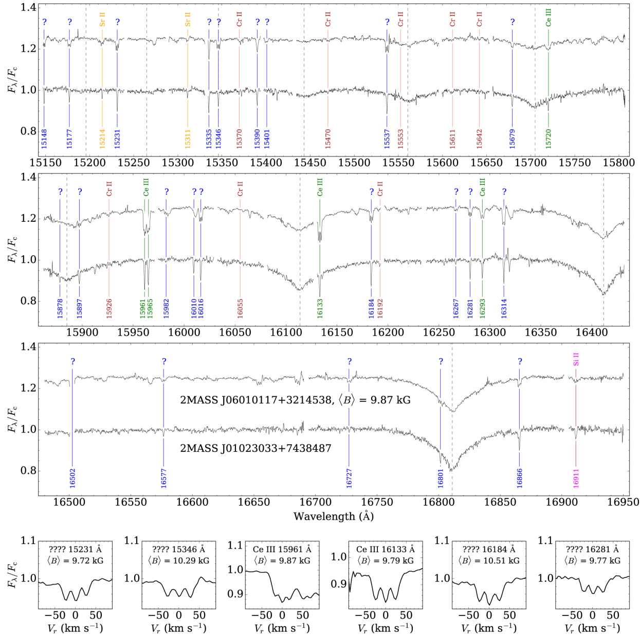
Figure 1. from Discovery of Resolved Magnetically Split Lines in SDSS/APOGEE Spectra of 157 Ap/Bp Stars null 2019 APJL 873 L5 doi:10.3847/2041-8213/ab0750 https://dx.doi.org/10.3847/2041-8213/ab0750
