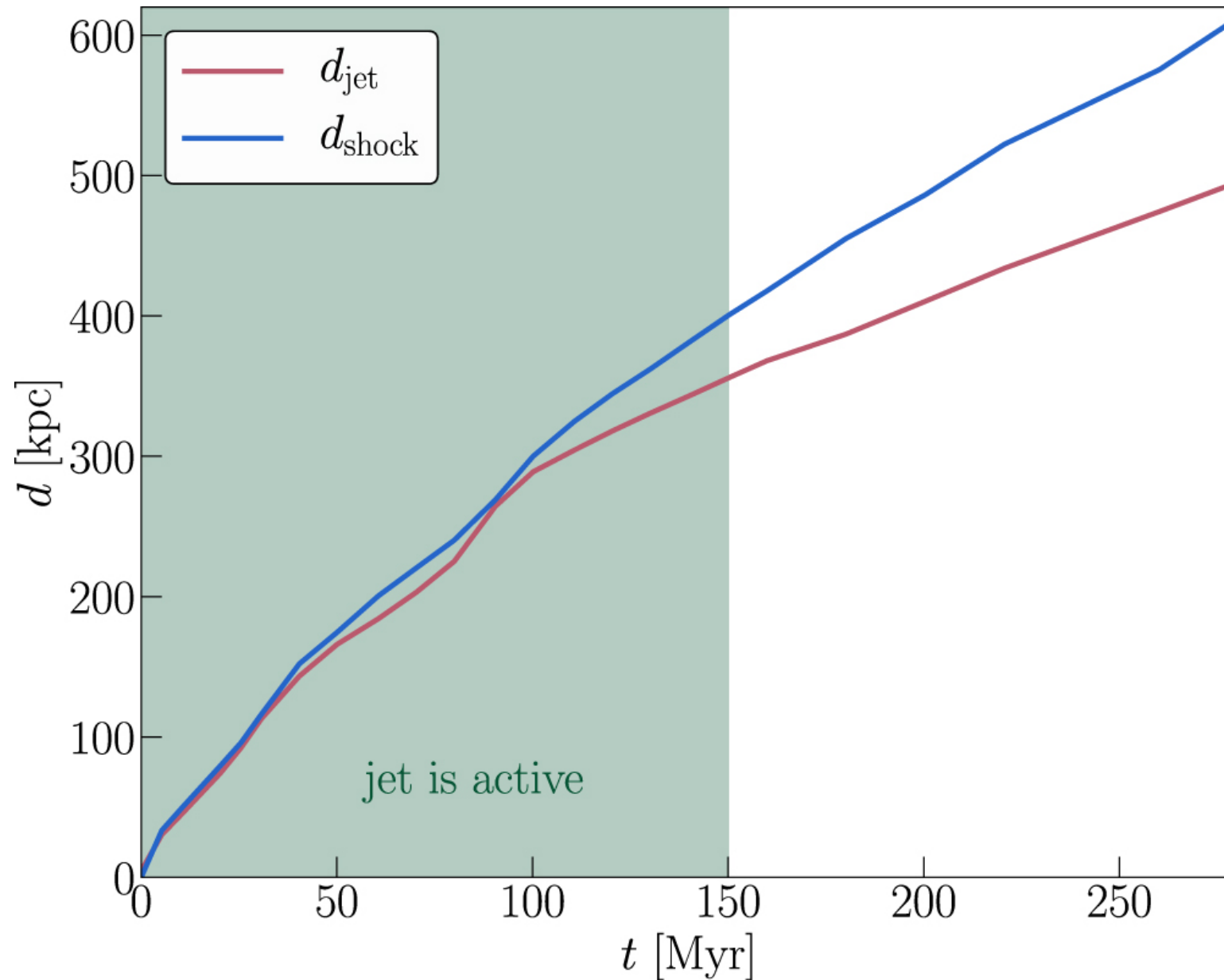
Figure 4. from The Sunyaev–Zel’dovich Effect of Simulated Jet-inflated Bubbles in Clusters null 2019 APJL 872 L8 doi:10.3847/2041-8213/ab020d https://dx.doi.org/10.3847/2041-8213/ab020d © 2019. The American Astronomical Society. All rights reserved.
