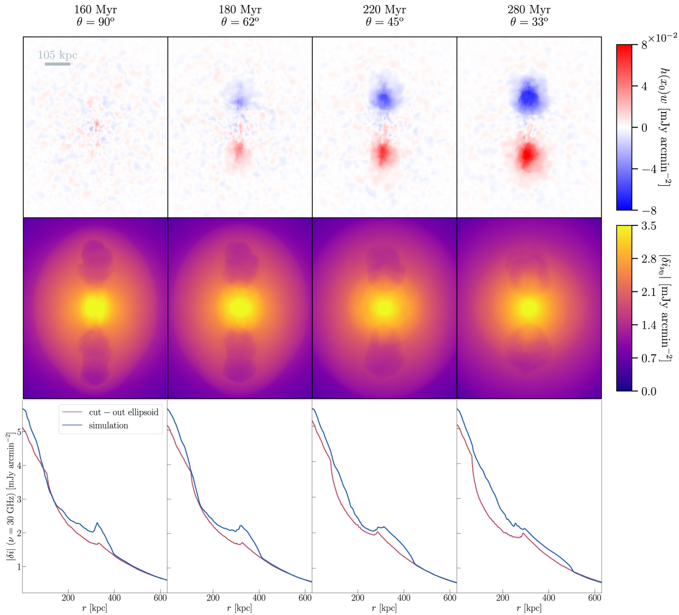
Figure 3. from The Sunyaev–Zel’dovich Effect of Simulated Jet-inflated Bubbles in Clusters null 2019 APJL 872 L8 doi:10.3847/2041-8213/ab020d http://dx.doi.org/10.3847/2041-8213/ab020d © 2019. The American Astronomical Society. All rights reserved.
