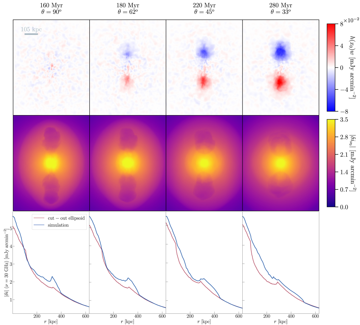
Figure 3. from The Sunyaev–Zel’dovich Effect of Simulated Jet-inflated Bubbles in Clusters null 2019 APJL 872 L8 doi:10.3847/2041-8213/ab020d https://dx.doi.org/10.3847/2041-8213/ab020d © 2019. The American Astronomical Society. All rights reserved.
