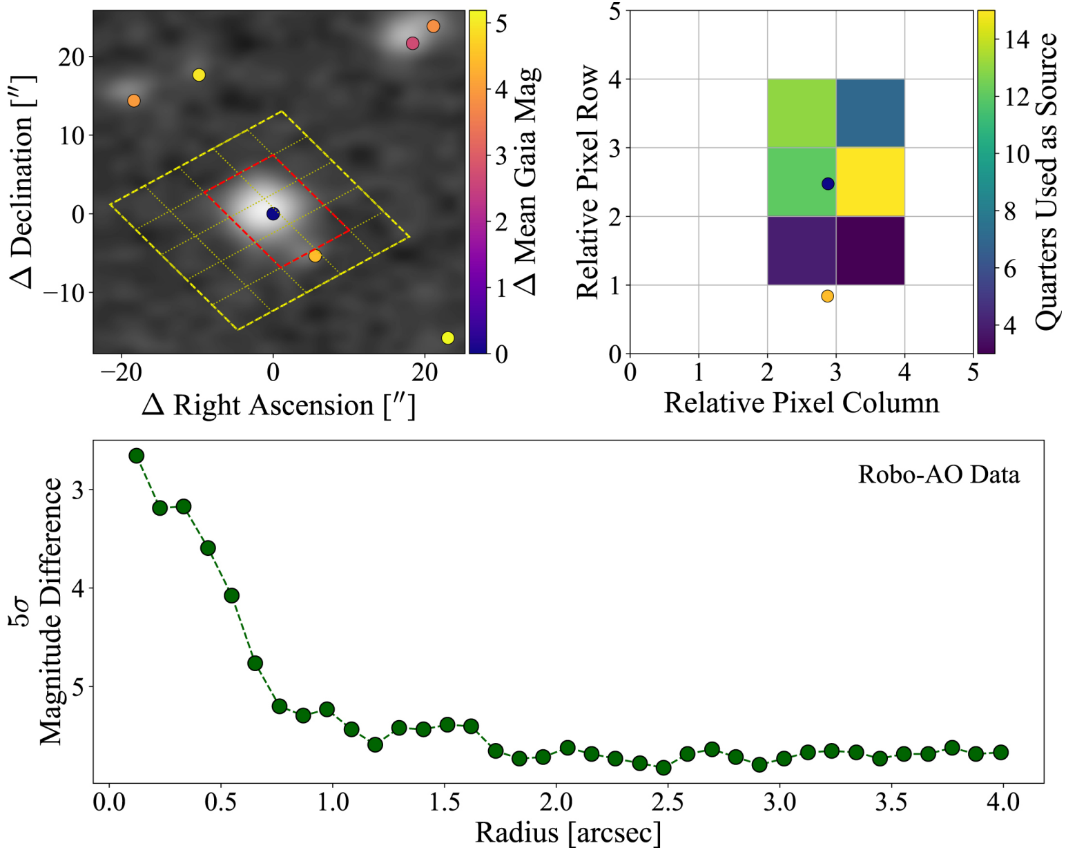
Figure 1. from Kepler-730: A Hot Jupiter System with a Close-in, Transiting, Earth-sized Planet null 2019 APJL 870 L17 doi:10.3847/2041-8213/aafa1e http://dx.doi.org/10.3847/2041-8213/aafa1e © 2019. The American Astronomical Society. All rights reserved.
