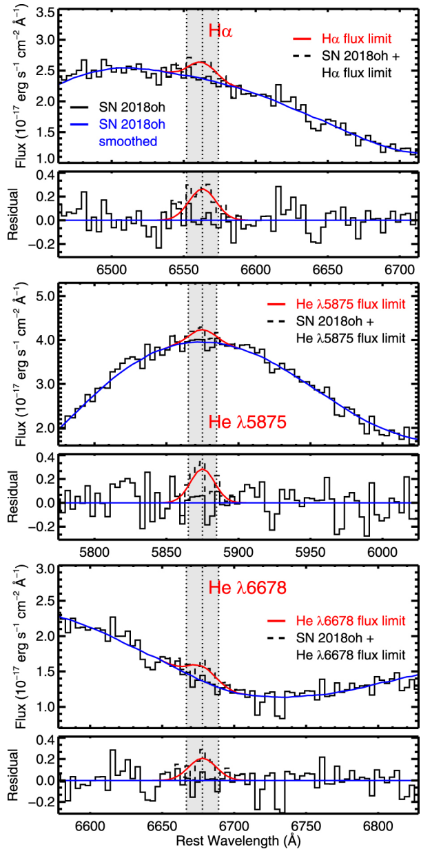
Figure 5. from Nebular Spectroscopy of Kepler's Brightest Supernova null 2019 APJL 870 L14 doi:10.3847/2041-8213/aaf9b1 http://dx.doi.org/10.3847/2041-8213/aaf9b1 © 2019. The American Astronomical Society. All rights reserved.
