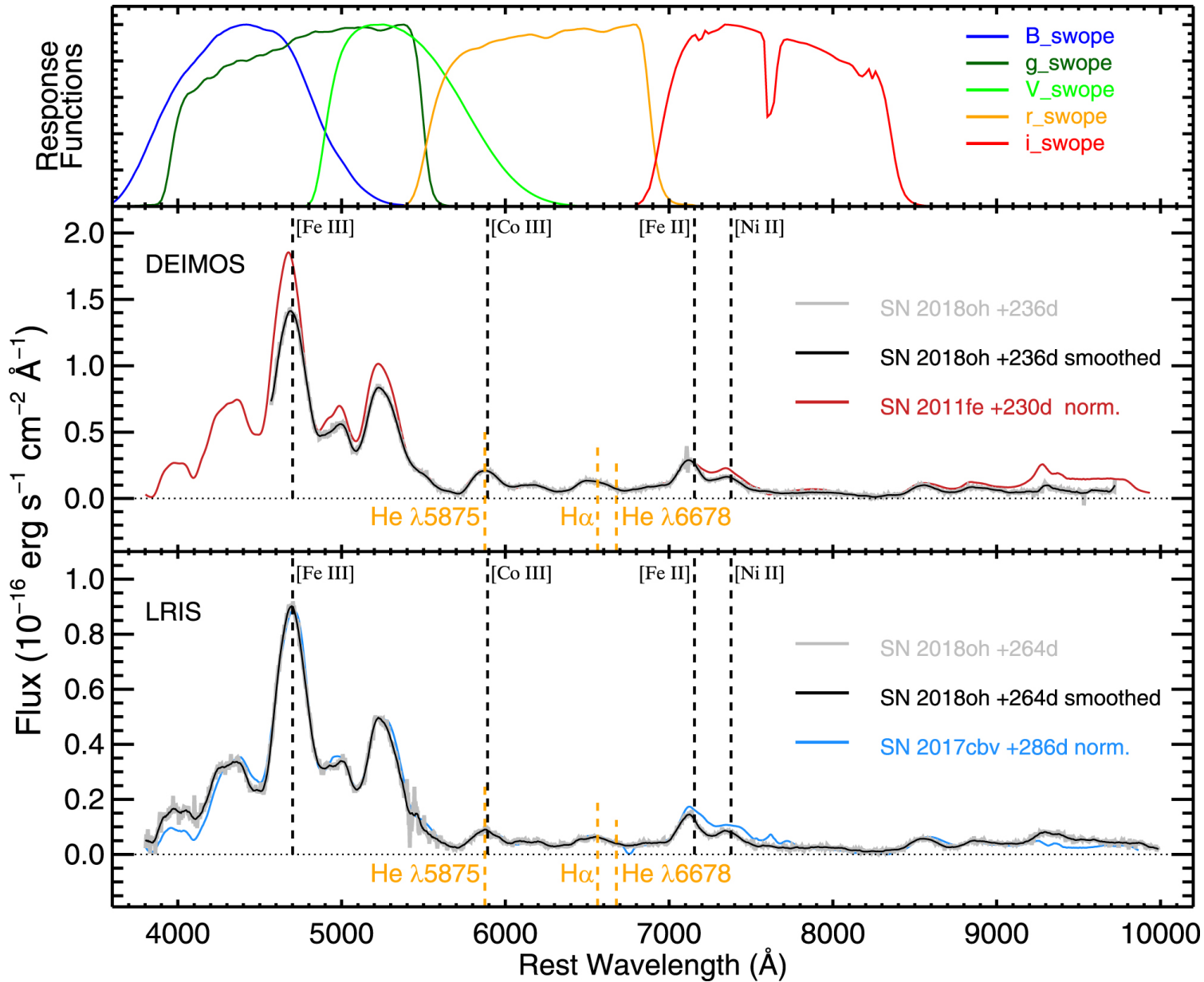
Figure 4. from Nebular Spectroscopy of Kepler's Brightest Supernova null 2019 APJL 870 L14 doi:10.3847/2041-8213/aaf9b1 http://dx.doi.org/10.3847/2041-8213/aaf9b1 © 2019. The American Astronomical Society. All rights reserved.
