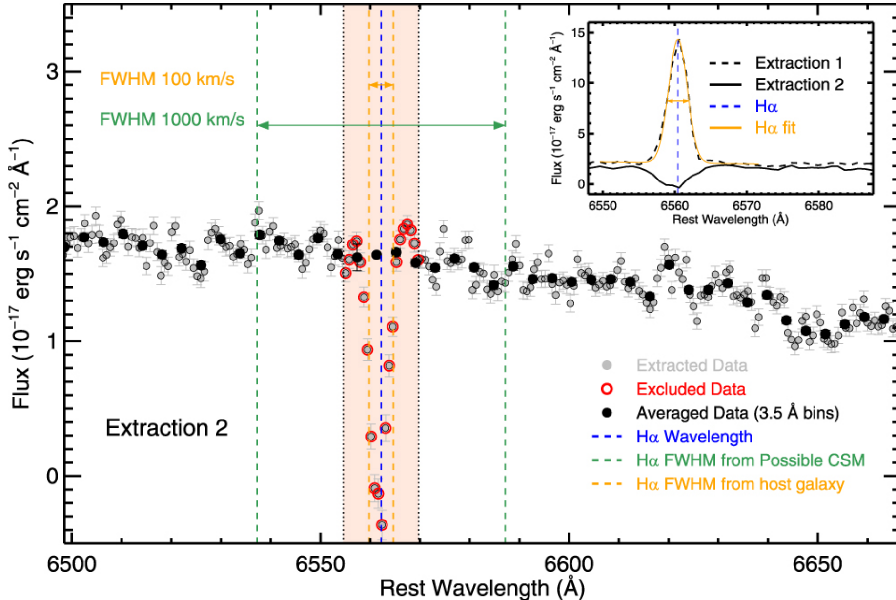
Figure 3. from Nebular Spectroscopy of Kepler's Brightest Supernova null 2019 APJL 870 L14 doi:10.3847/2041-8213/aaf9b1 http://dx.doi.org/10.3847/2041-8213/aaf9b1 © 2019. The American Astronomical Society. All rights reserved.
