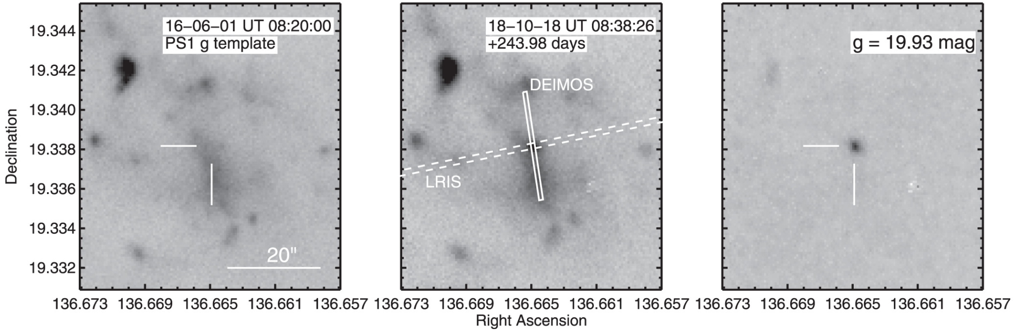
Figure 1. from Nebular Spectroscopy of Kepler's Brightest Supernova null 2019 APJL 870 L14 doi:10.3847/2041-8213/aaf9b1 http://dx.doi.org/10.3847/2041-8213/aaf9b1 © 2019. The American Astronomical Society. All rights reserved.
