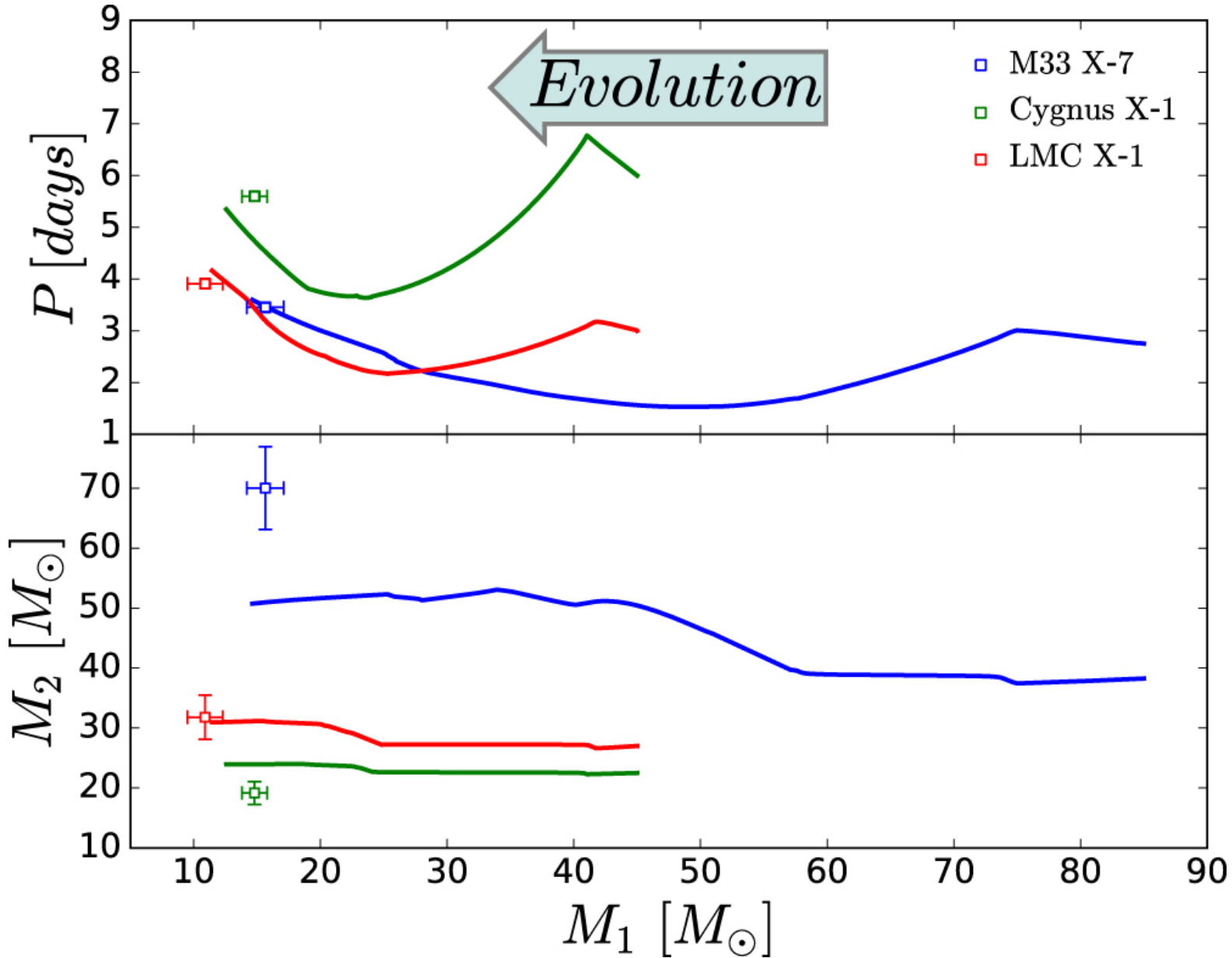
Figure 5. from On the Origin of Black Hole Spin in High-mass X-Ray Binaries null 2019 APJL 870 L18 doi:10.3847/2041-8213/aaf97b http://dx.doi.org/10.3847/2041-8213/aaf97b © 2019. The American Astronomical Society. All rights reserved.
