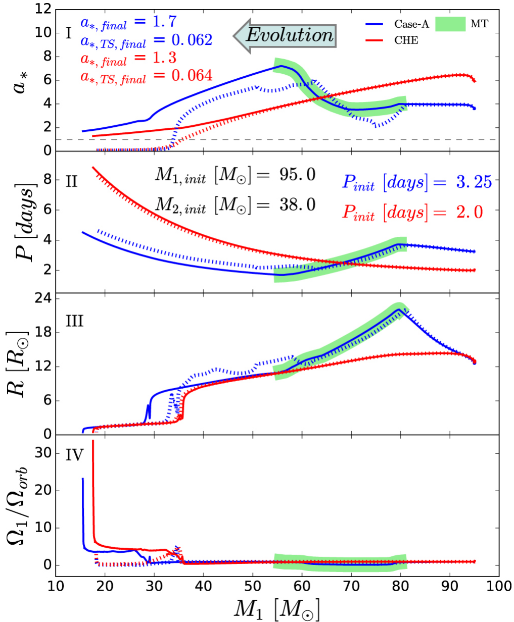
Figure 1. from On the Origin of Black Hole Spin in High-mass X-Ray Binaries null 2019 APJL 870 L18 doi:10.3847/2041-8213/aaf97b http://dx.doi.org/10.3847/2041-8213/aaf97b © 2019. The American Astronomical Society. All rights reserved.
