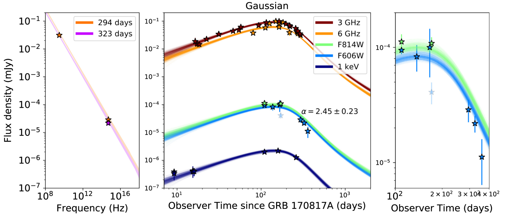
Figure 3. from The Optical Afterglow of GW170817 at One Year Post-merger null 2019 APJL 870 L15 doi:10.3847/2041-8213/aaf96b http://dx.doi.org/10.3847/2041-8213/aaf96b © 2019. The American Astronomical Society. All rights reserved.
