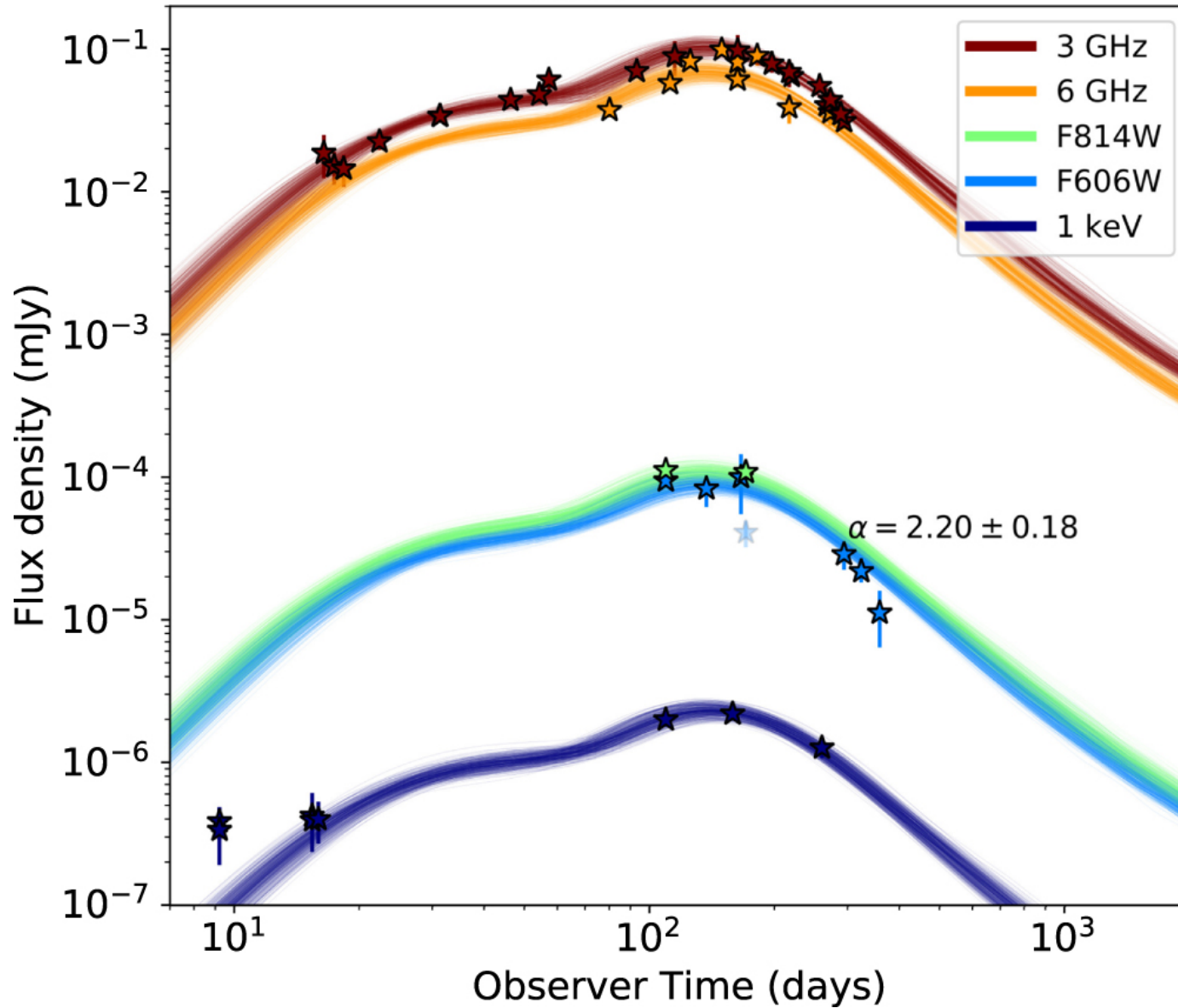
Figure 2. from The Optical Afterglow of GW170817 at One Year Post-merger null 2019 APJL 870 L15 doi:10.3847/2041-8213/aaf96b http://dx.doi.org/10.3847/2041-8213/aaf96b © 2019. The American Astronomical Society. All rights reserved.
