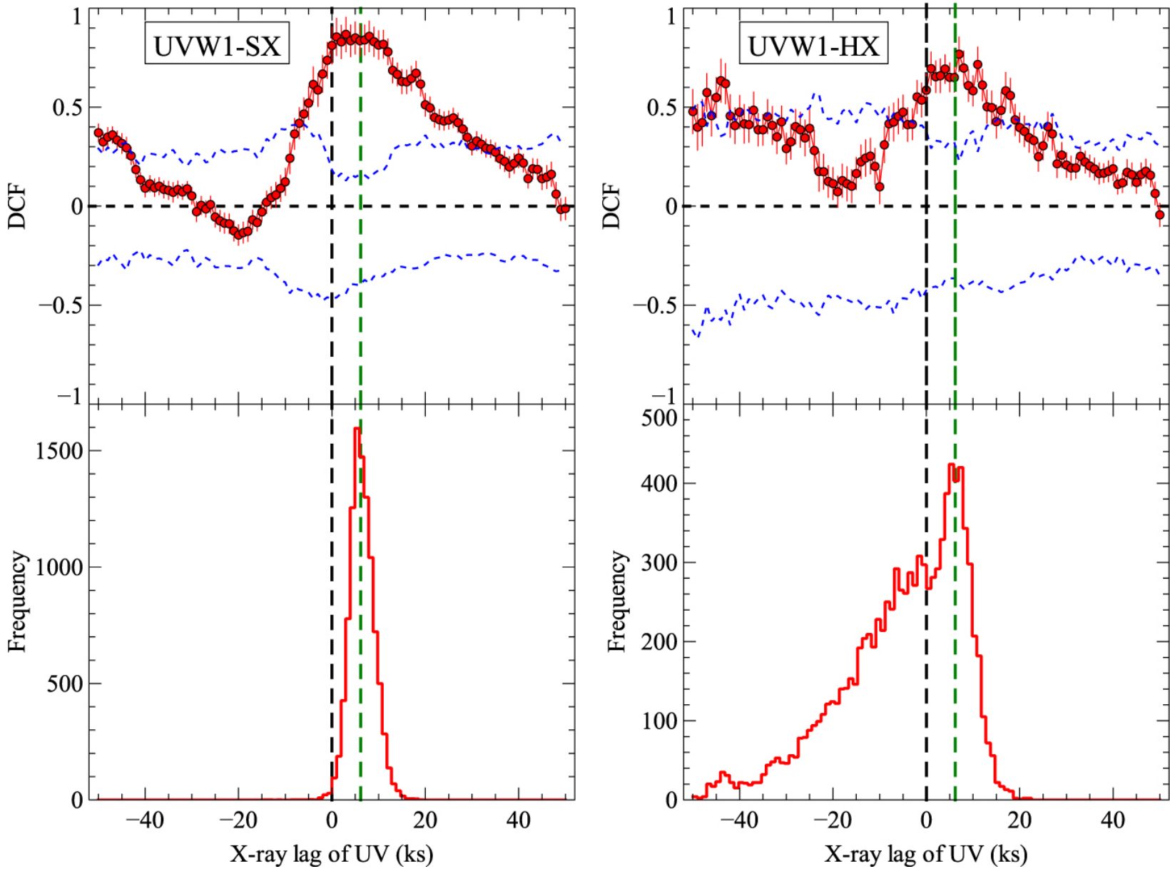
Figure 3. from UV to X-Ray Comptonization Delay in Mrk 493 null 2019 APJL 870 L13 doi:10.3847/2041-8213/aaf8ab http://dx.doi.org/10.3847/2041-8213/aaf8ab © 2019. The American Astronomical Society. All rights reserved.
